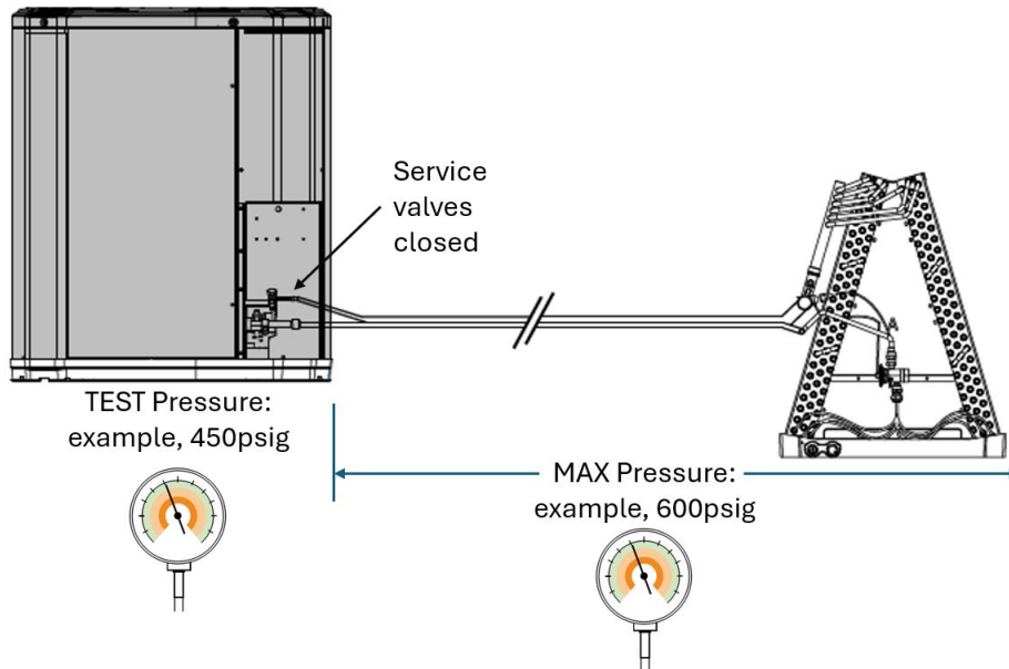
Figure 27. Check for leaks
