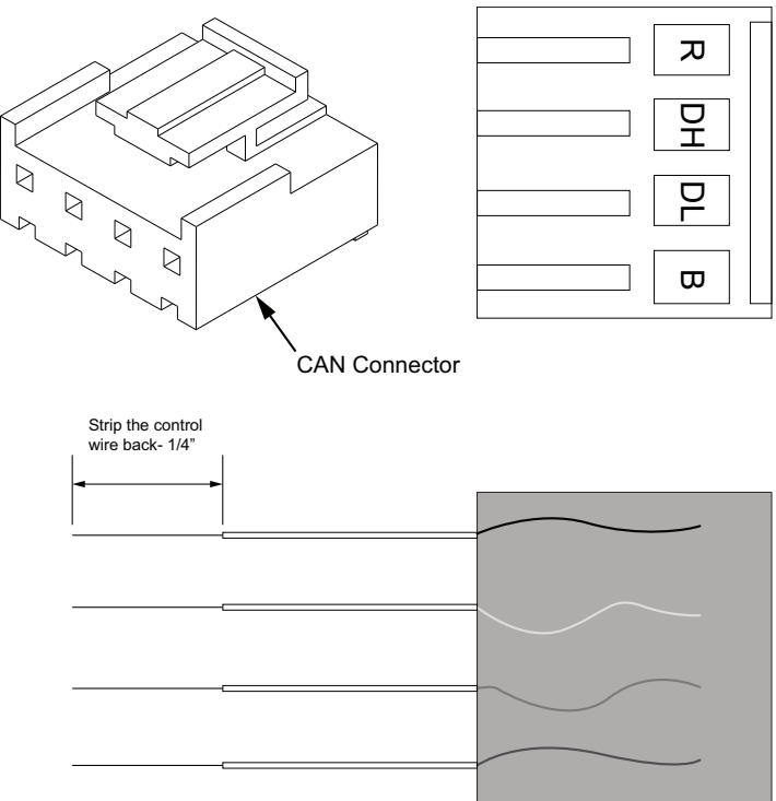
Figure 33. For use with 18 gauge solid core thermostat wire
