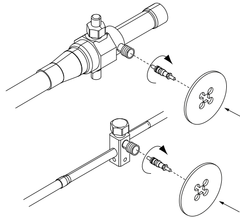
Figure 25. Re-installation of pressure valve cores and plastic tabs
