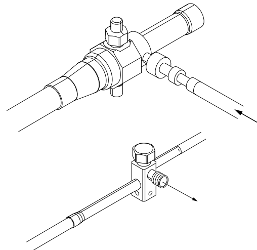
Figure 23. Purging of refrigerant lines
