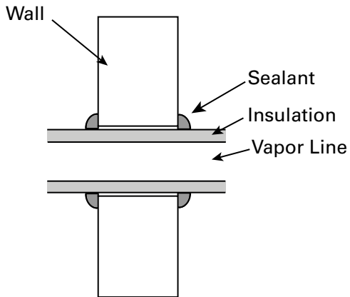
Figure 20. Incorrect lineset installation
