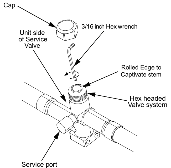
Figure 31. Liquid service valve
