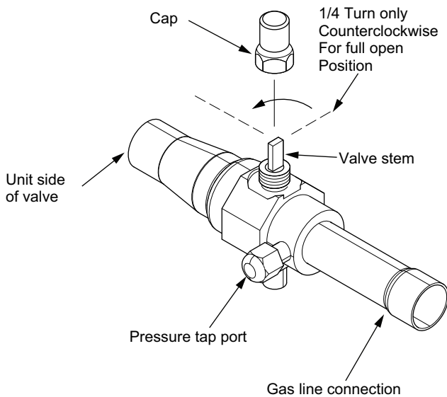
Figure 30. Gas service valve
