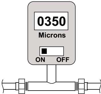
Figure 28. Observe micron gauge reading
