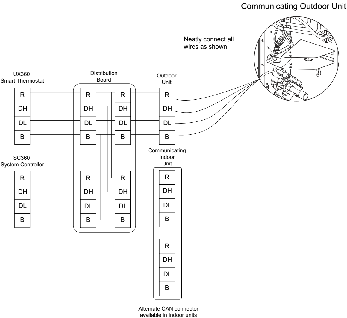
Figure 32. Low-voltage connection diagrams in Link mode
