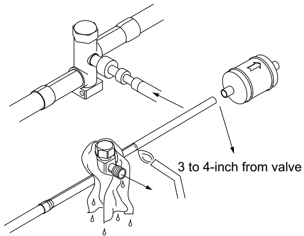
Figure 24. Wrapping of wet rag
