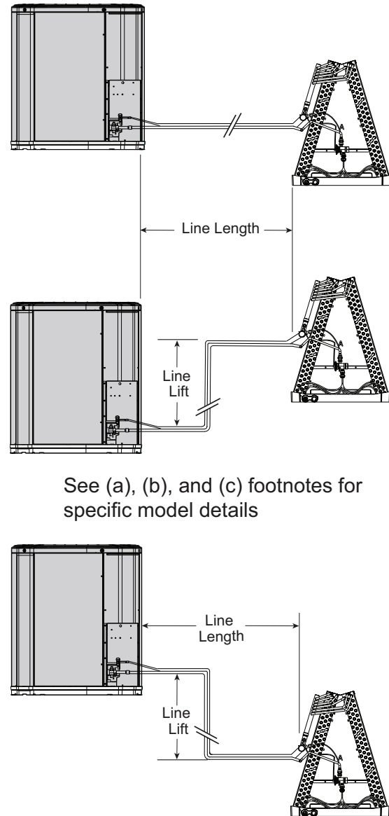
Figure 3. Example of line lift and length
