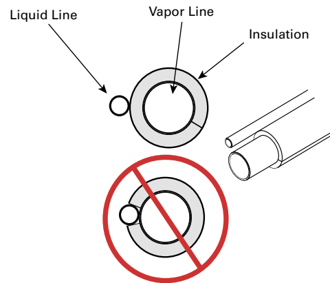
Figure 15. Refrigerant line insulation
