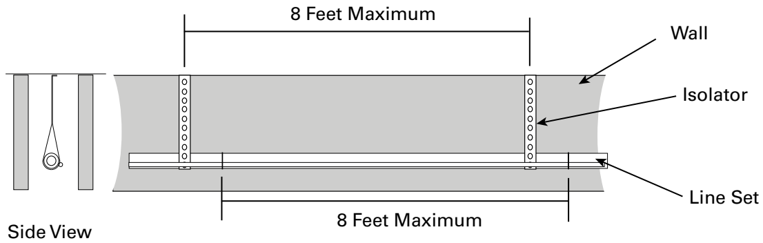
Figure 18. Isolation in wall spaces
