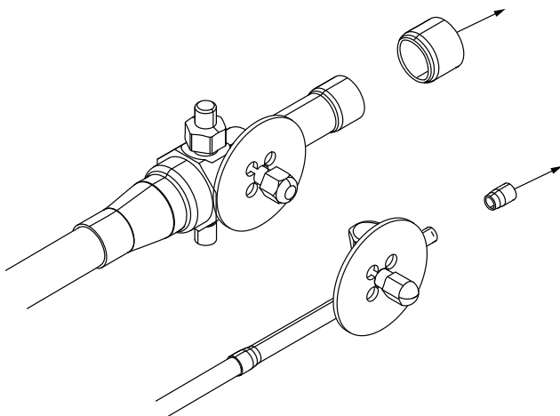
Figure 21. Removal of caps or plugs from pipe ends
