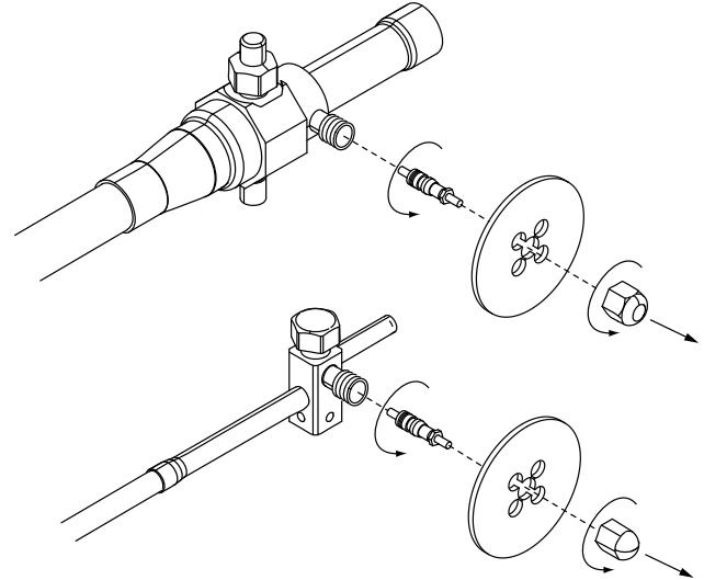
Figure 23. Purging of refrigerant lines
