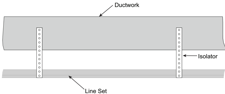
Figure 20. Incorrect lineset installation
