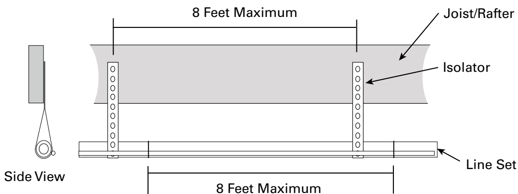
Figure 17. Isolation from a joist/rafter
