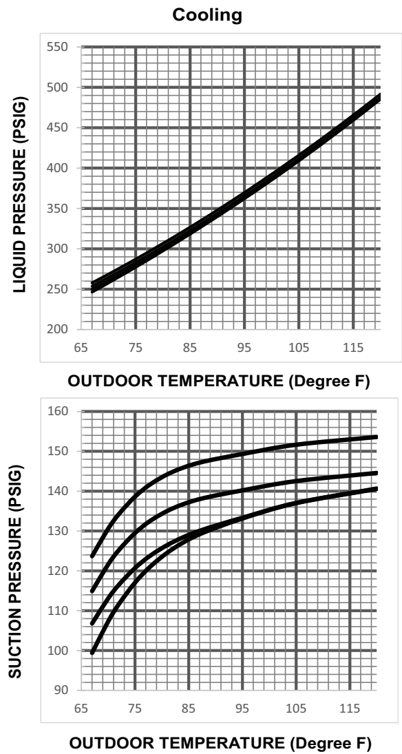
Figure 34. 4 ton AC (X48 model)
