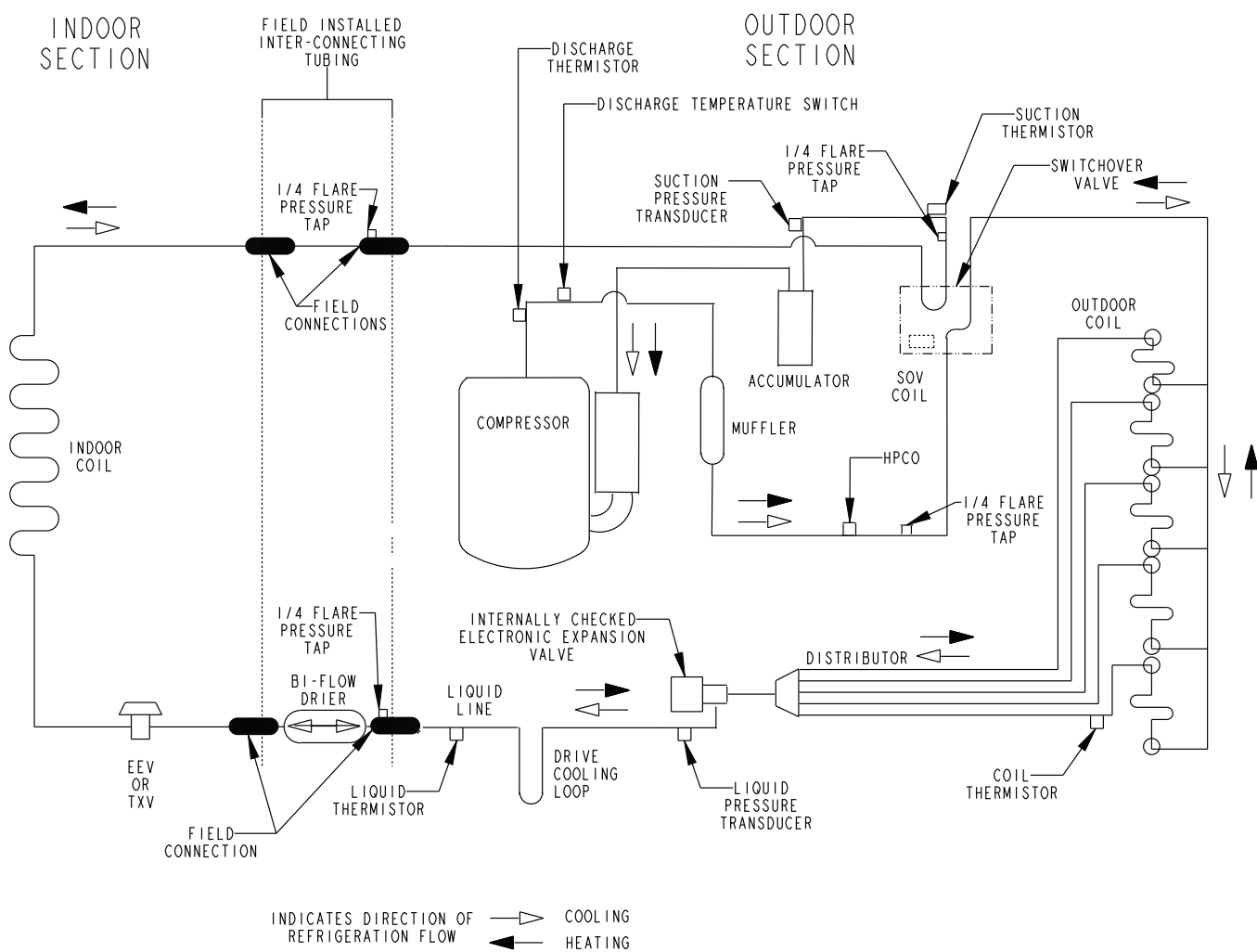
Figure 15. 2-ton and 3-ton HP (X24 and X36 models)
