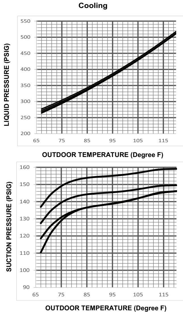
Figure 33. 3 ton AC (X36 model)
