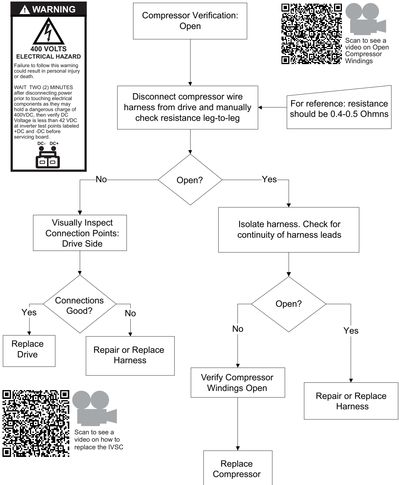
Figure 23. Compressor verification: open flowchart
