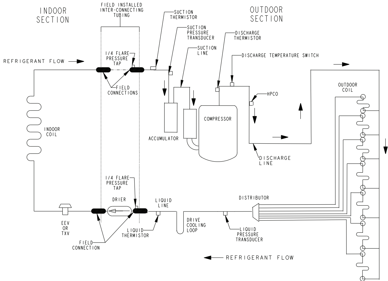
Figure 14. 4-ton and 5-ton AC (X48 and X60 models)
