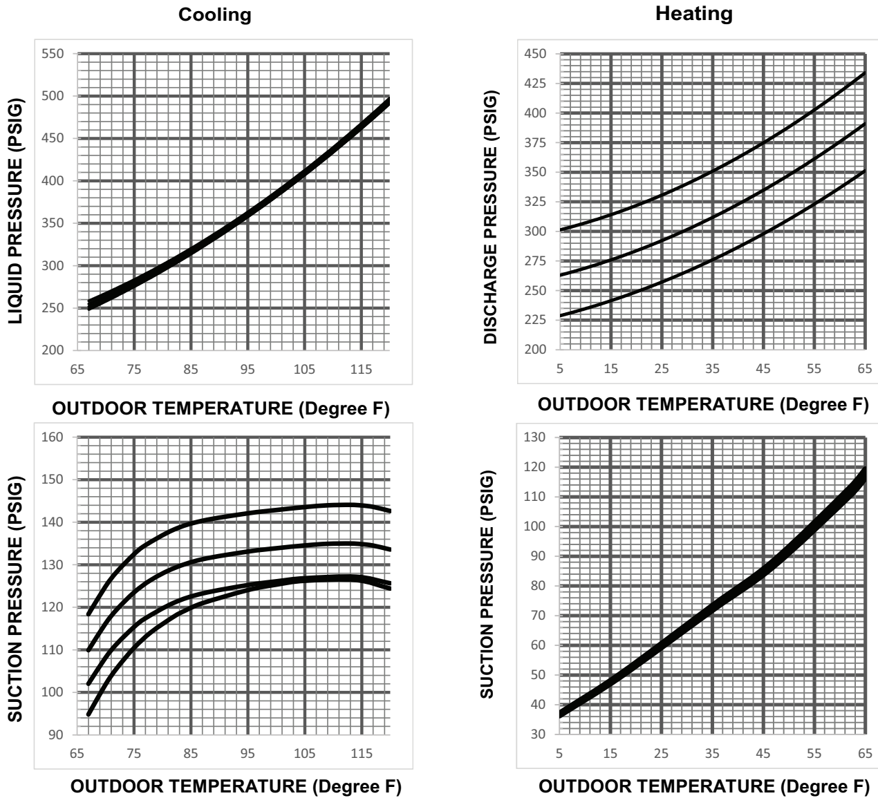
Figure 31. 5 ton HP (X60 model)
