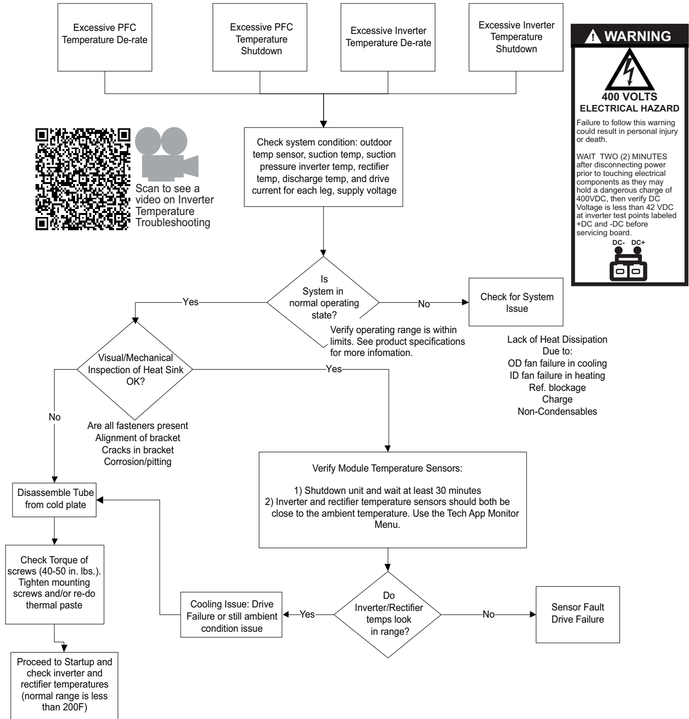
Figure 24. Inverter temperature flowchart
