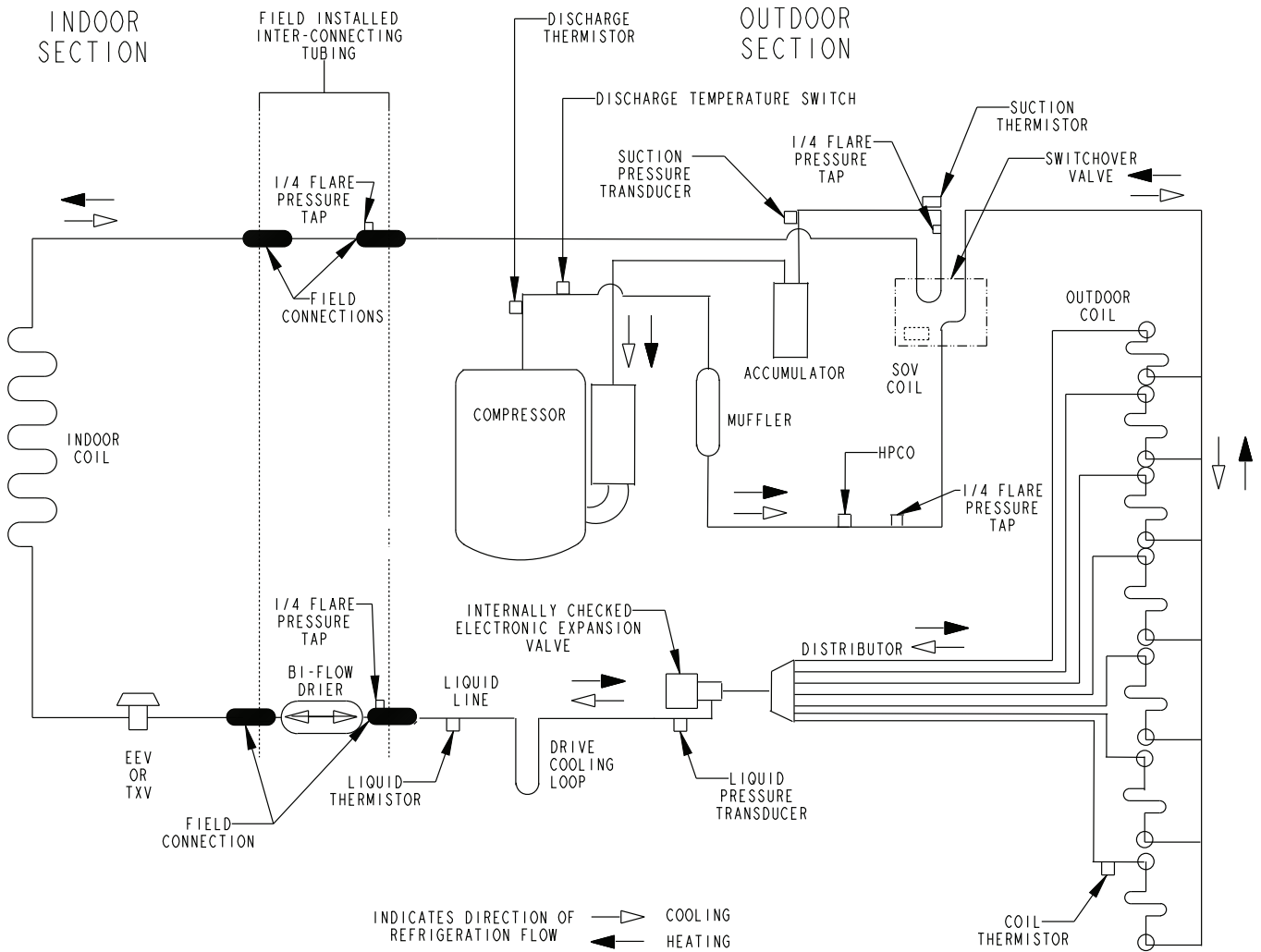
Figure 16. 4-ton and 5-ton HP (X48 and X60 models)
