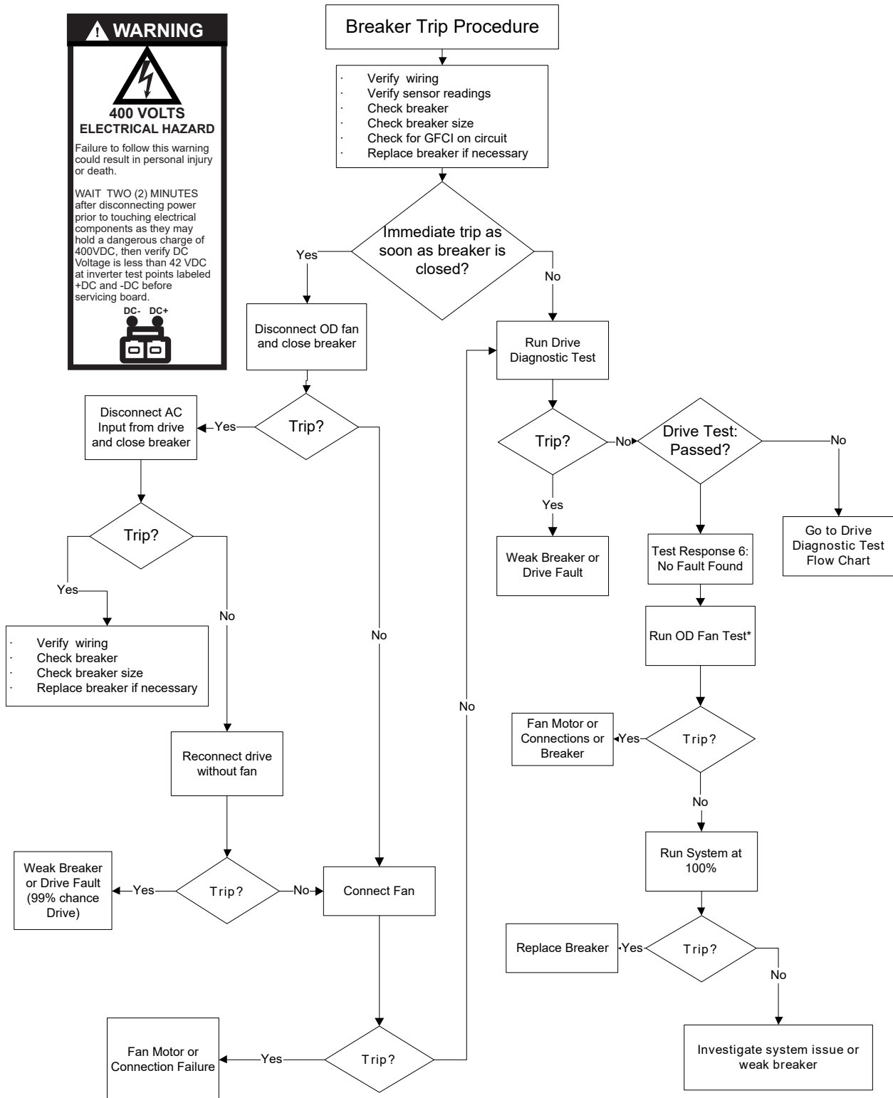
Figure 19. Breaker trip procedure flowchart
