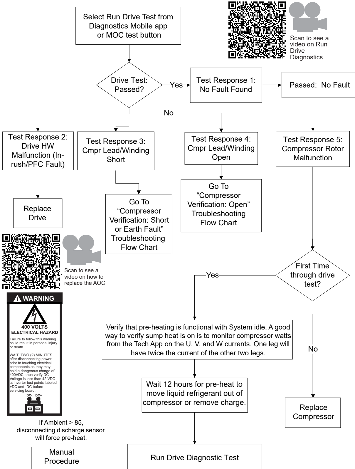
Figure 21. Run drive diagnostic test flowchart
