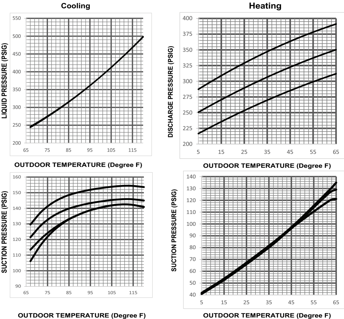
Figure 28. 2 ton HP (X24 model)
