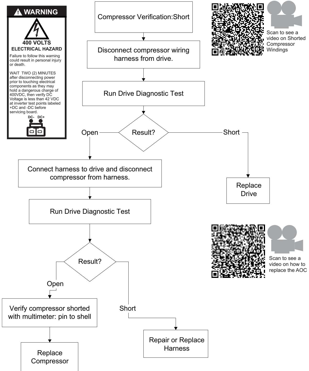
Figure 22. Compressor verification: short flowchart
