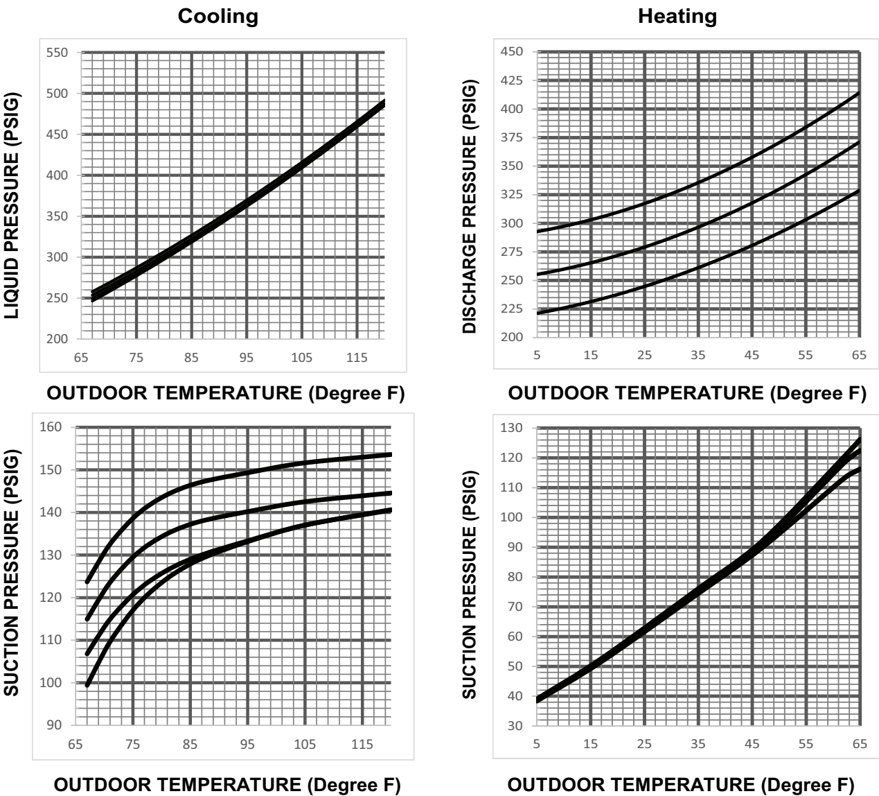
Figure 30. 4 ton HP (X48 model)
