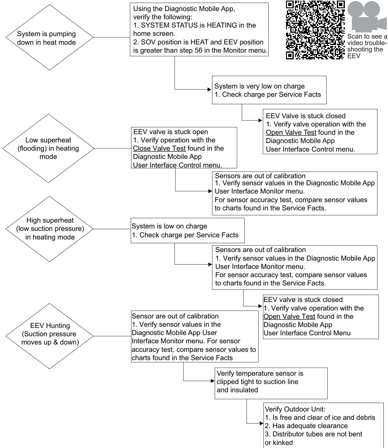
Figure 26. EEV troubleshooting flowchart
