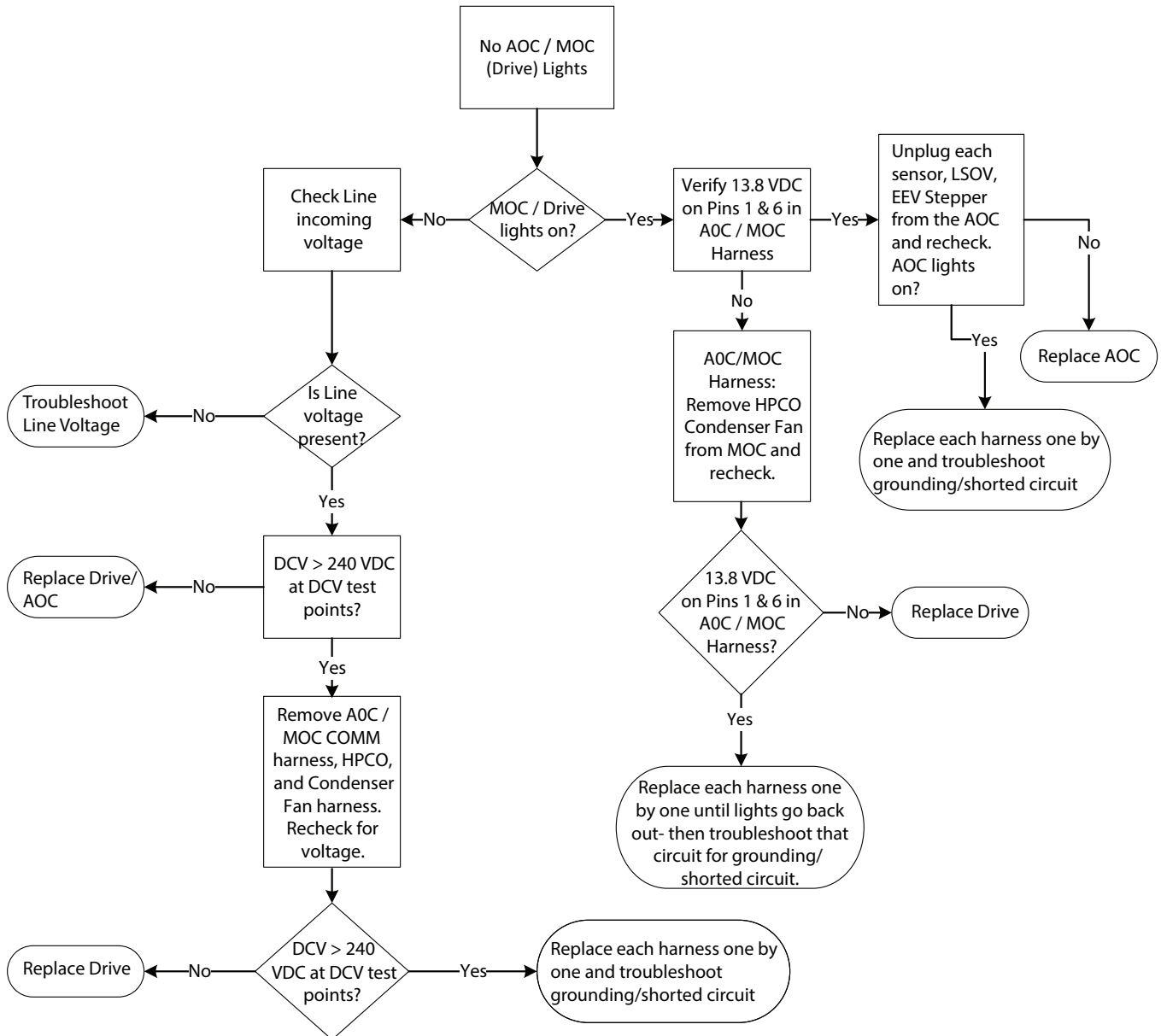
Figure 18. Communication loss flowchart
