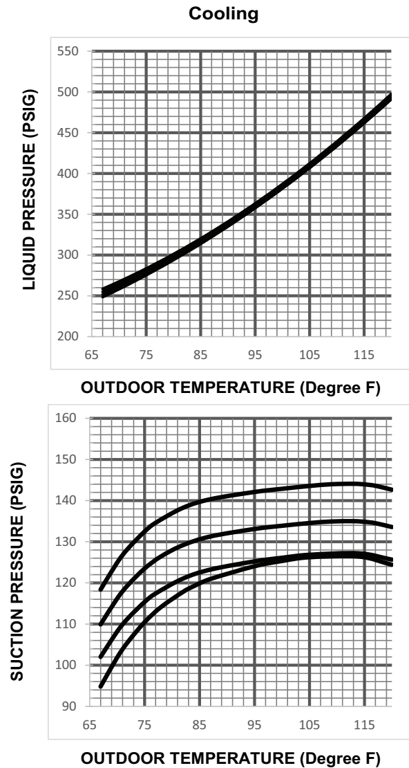
Figure 35. 5 ton AC (X60 model)
