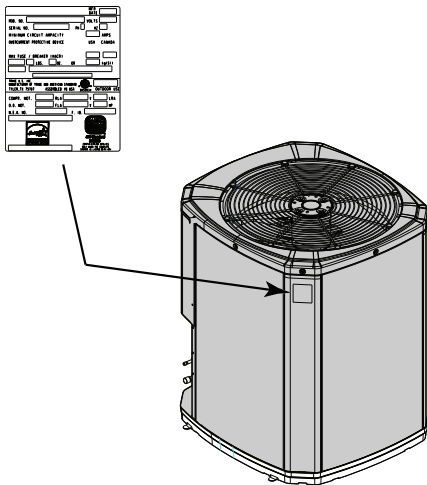
Figure 7. Equipment nameplate
