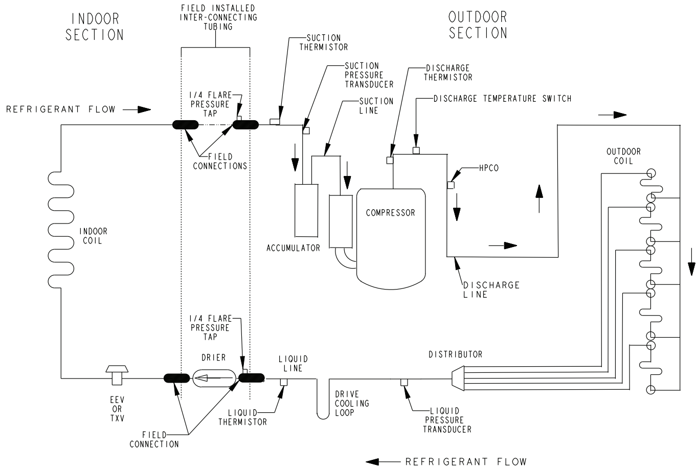
Figure 13. 2-ton and 3-ton AC (X24 and X36 models)
