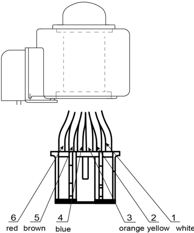
Figure 25. Stepper motor troubleshooting
