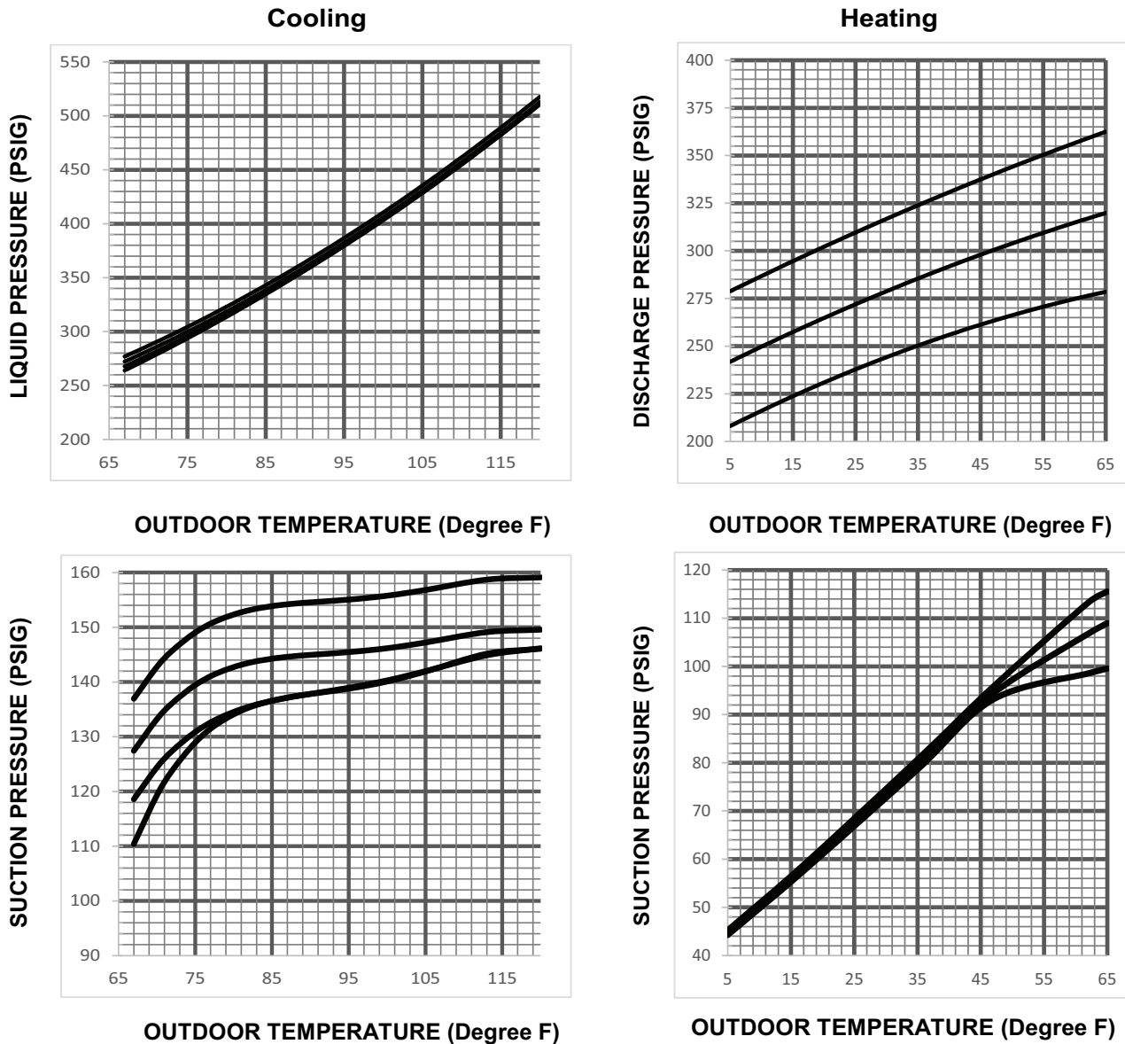
Figure 29. 3 ton HP (X36 model)
