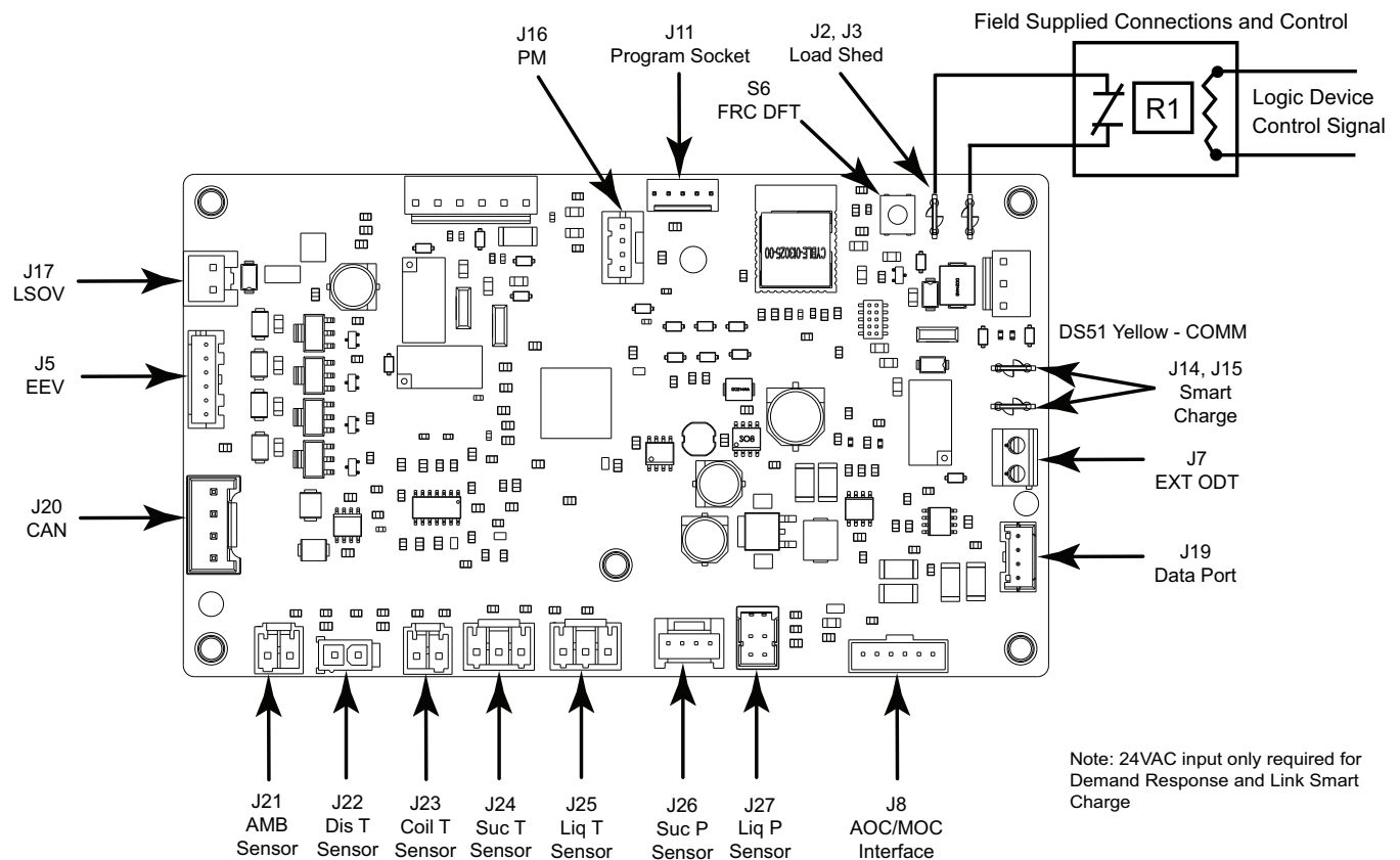
Figure 17. Load shed AOC diagram
