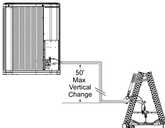
Figure 3. Refrigerant piping vertical change limit
