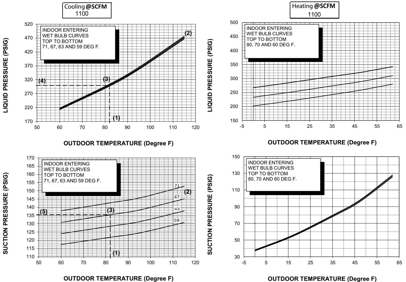
Figure 49. Pressure curves – model 5A6C4036A
