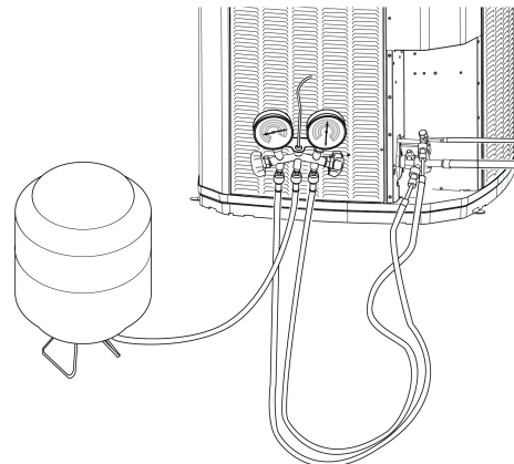
Figure 40. Charging the unit
