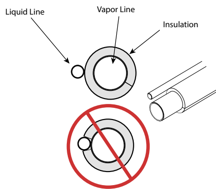
Figure 6. Refrigerant line insulation
