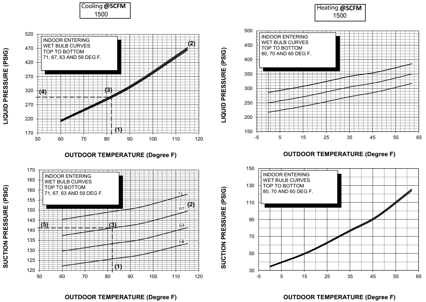
Figure 52. Pressure curves – model 5A6C4060A
