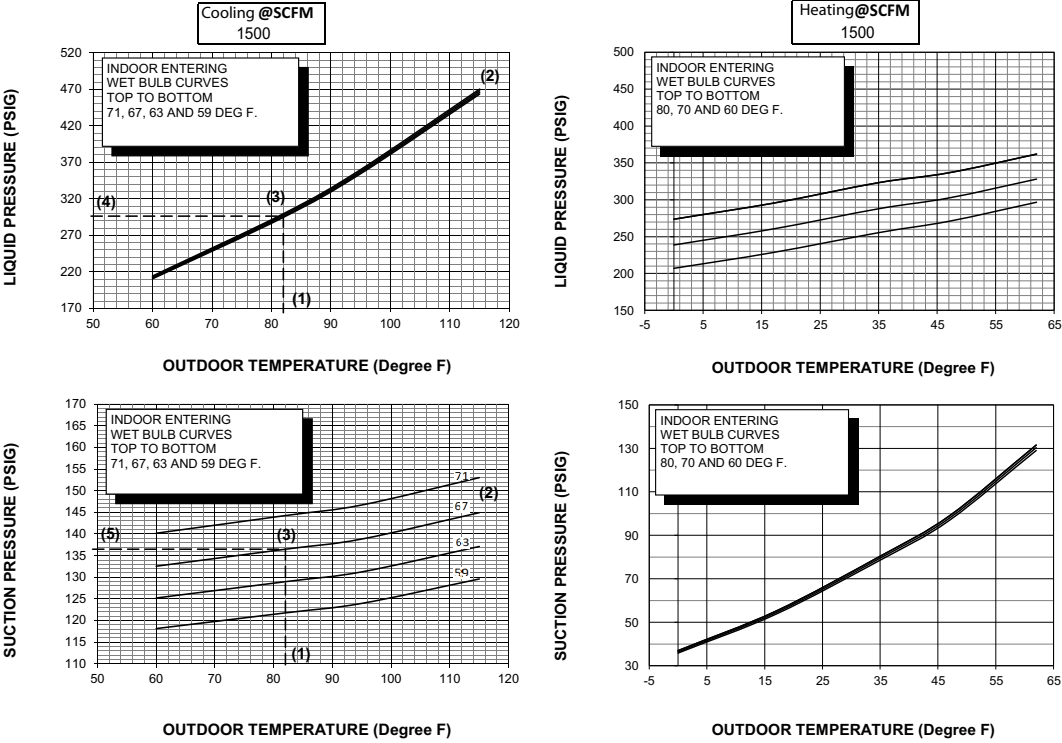
Figure 51. Pressure curves – model 5A6C4048A
