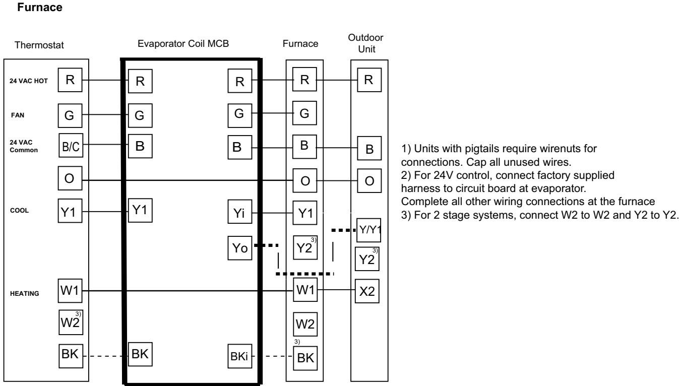
Figure 24. AC or heat pump, typical (with furnace)
