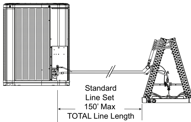
Figure 2. Refrigerant piping vertical change limit
