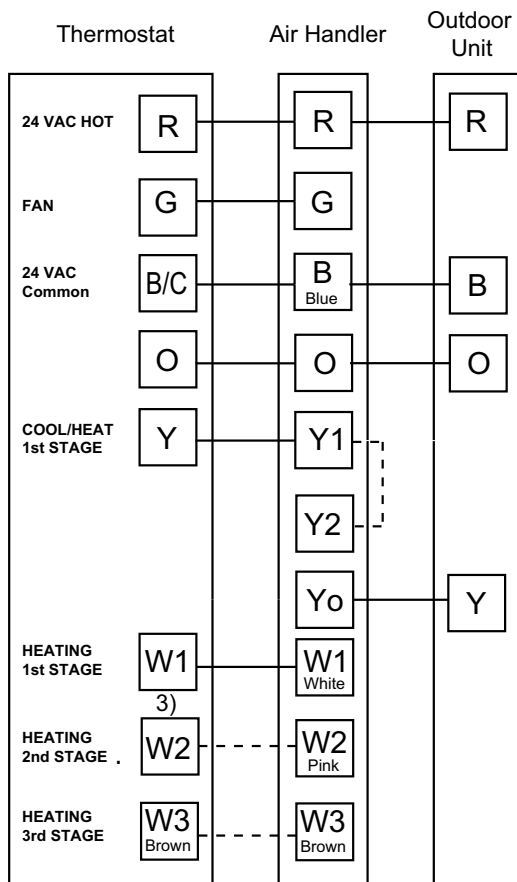
Figure 23. Single-stage, HP, 5TAM5
