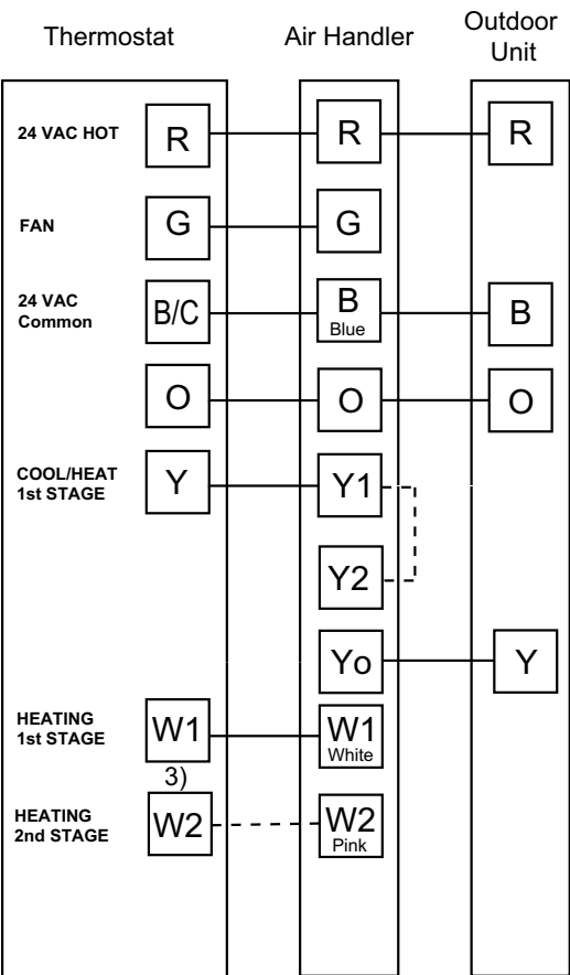
Figure 22. Single-stage, HP, 5TEM4
