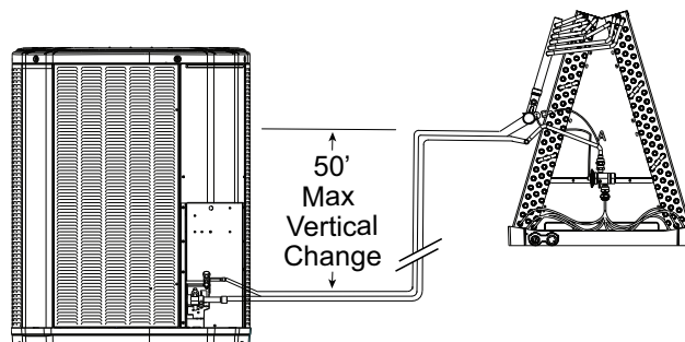
Figure 3. Refrigerant piping vertical change limit
