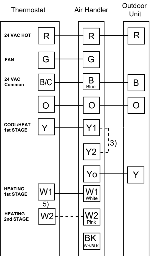
Figure 21. Single-stage, HP, 5TEM6
