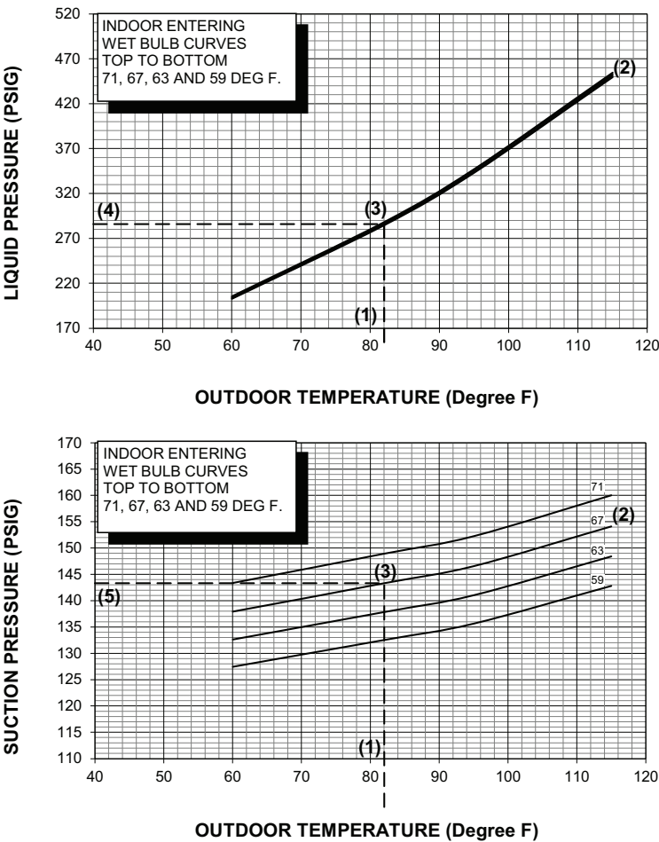
Figure 37. Pressure curves - model 5A7A5018A1
