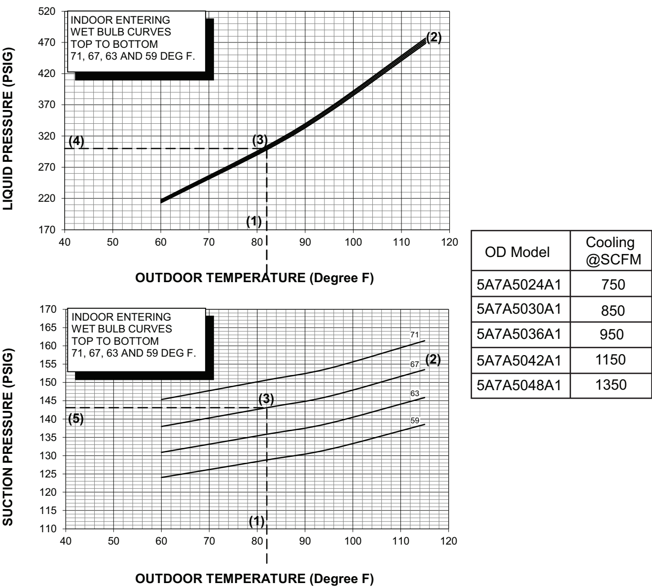
Figure 38. Pressure curves - model 5A7A5024A1, 5A7A5030A1, 5A7A5036A1, 5A7A5042A1, and 5A7A5048A1
