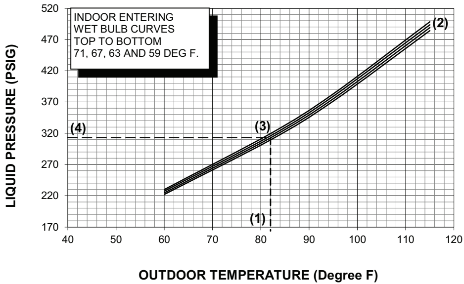
Figure 39. Pressure curves - model 5A7A5060A1
