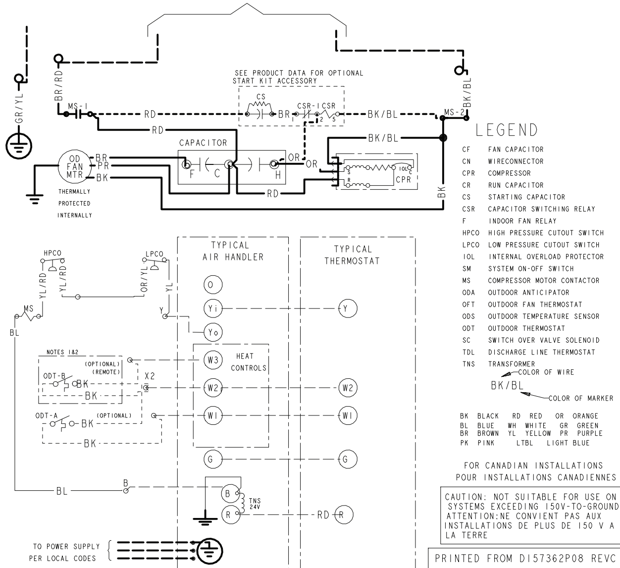
Figure 1. Models — 5A7A4018A, 024A, 030A, 036A, 042A, and 048A
