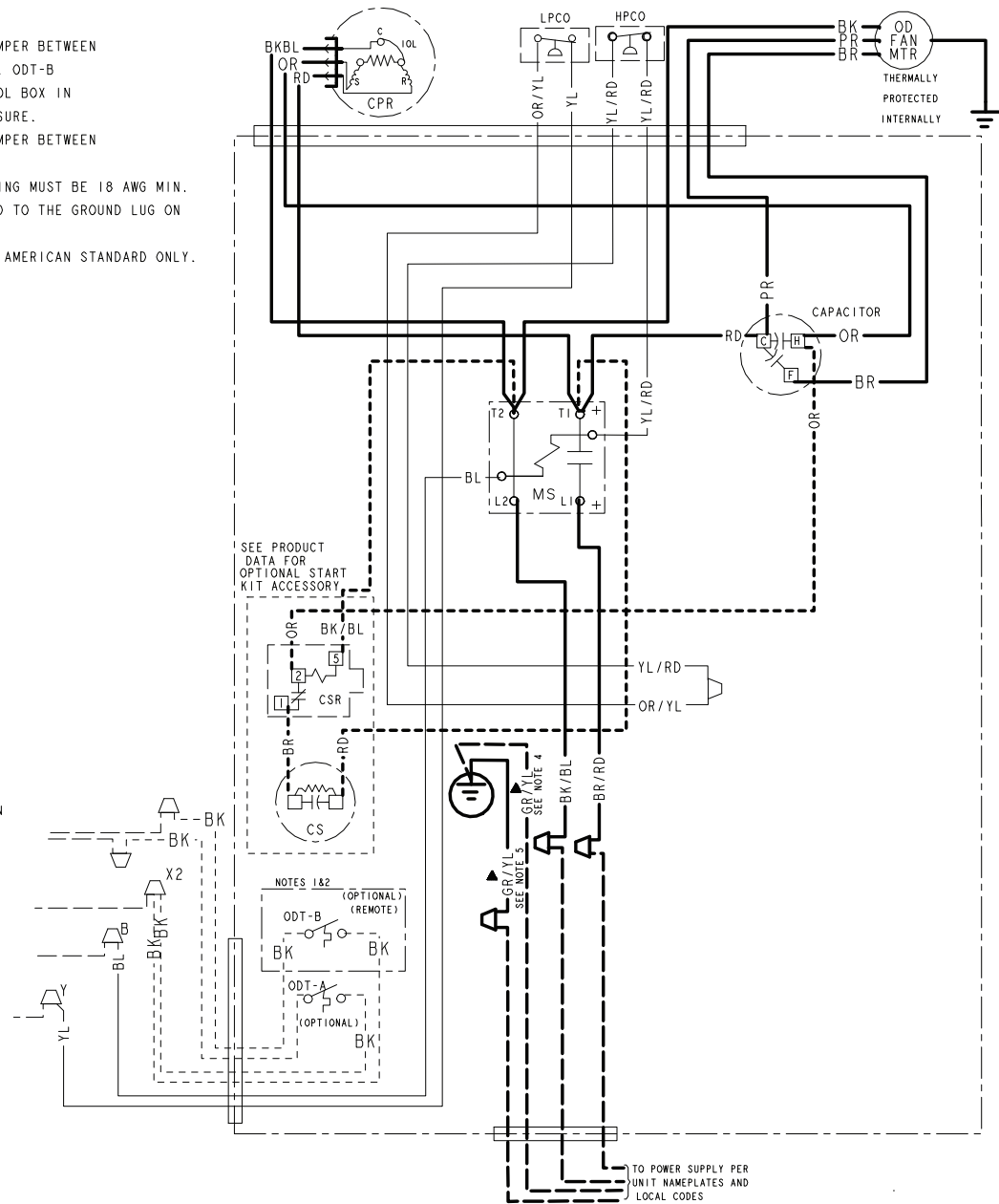
Figure 2. Models — 5A7A4018A, 024A, 030A, 036A, 042A, and 048A
