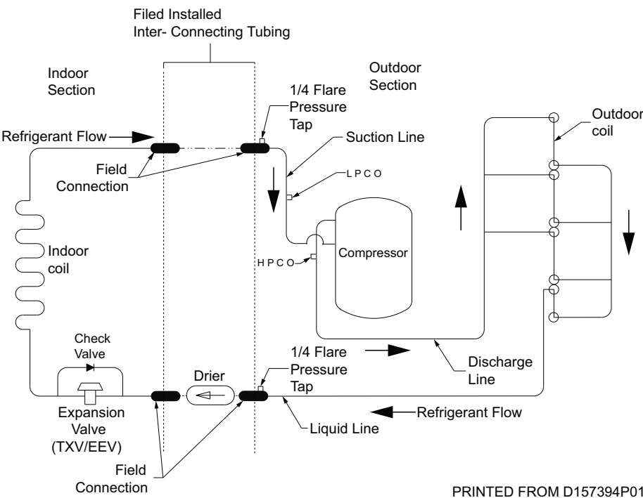
Figure 40. Refrigeration cycle for models 024 and 036
