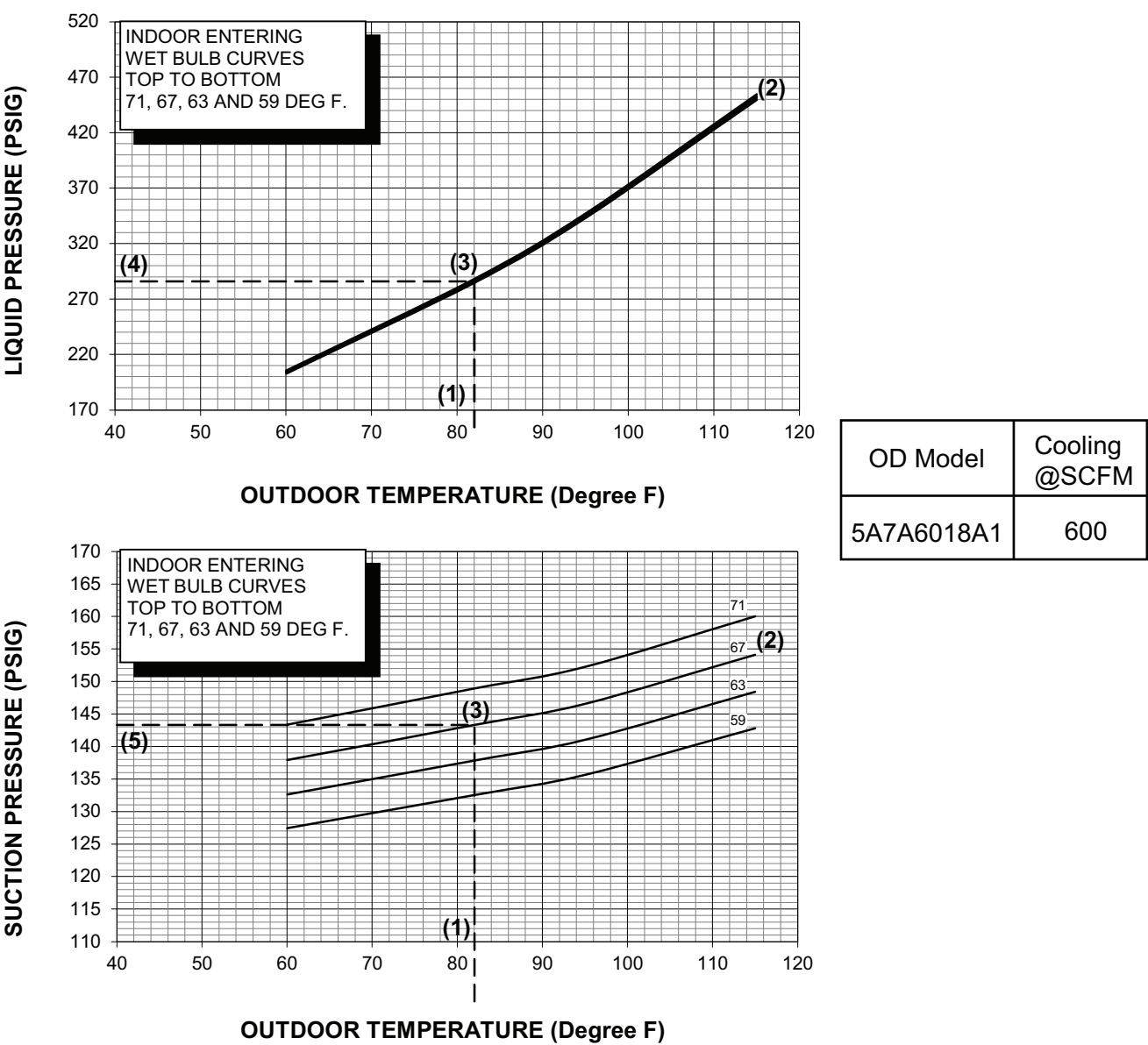
Figure 36. Pressure curves - model 5A7A6018A1
