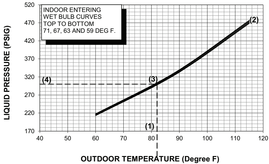
Figure 37. Pressure curves - model 5A7A6024A1, 5A7A6030A1, 5A7A6036A1, 5A7A6042A1, and 5A7A6048A1
