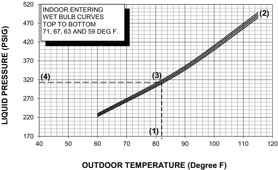
Figure 38. Pressure curves - model 5A7A6060A1
