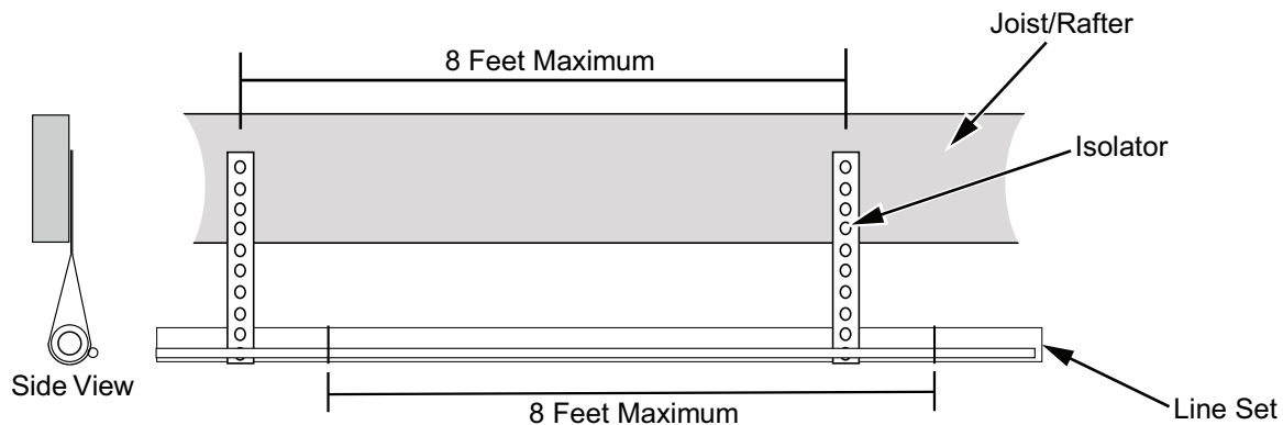
Figure 7. Isolation from joist/rafter
