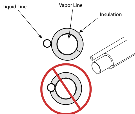
Figure 5. Refrigerant line insulation
