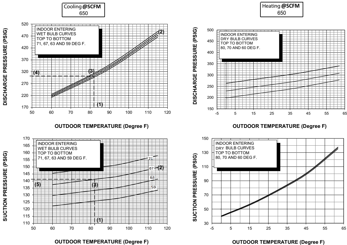
Figure 40. Pressure curves - model 5A6H4018A1
