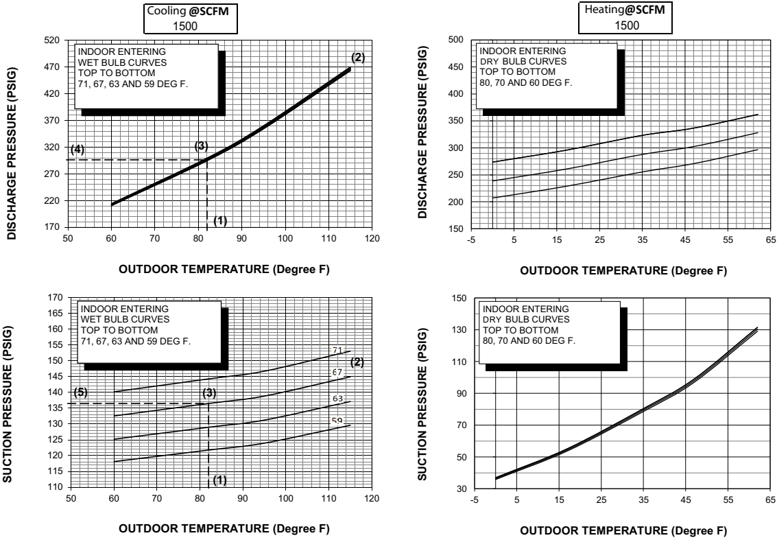
Figure 46. Pressure curves - model 5A6H4060A1
