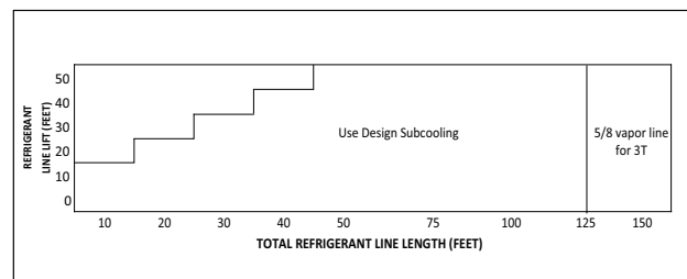
Figure 30. Subcool charging chart - models 018A, 024A, 030A, and 036A
