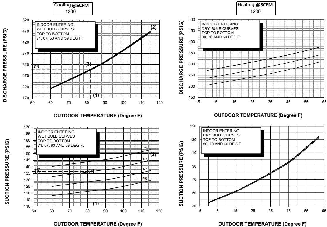
Figure 44. Pressure curves - model 5A6H4042A1
