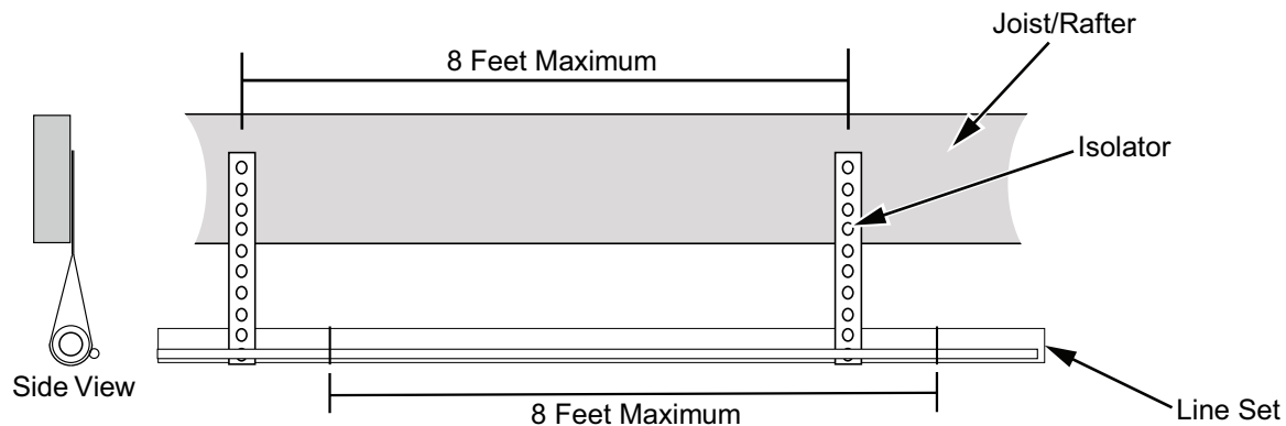
Figure 6. Isolation from joist/rafter
