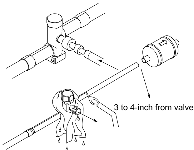
Figure 13. Wrapping of wet rag
