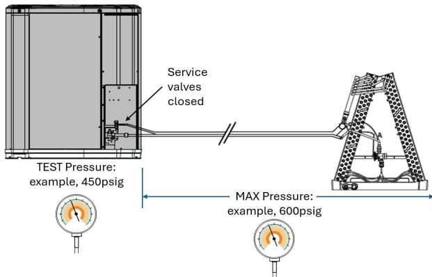
Figure 15. Refrigerant line leak check
