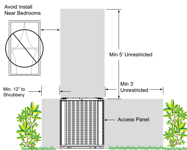
Figure 4. Suggested locations for best reliability
