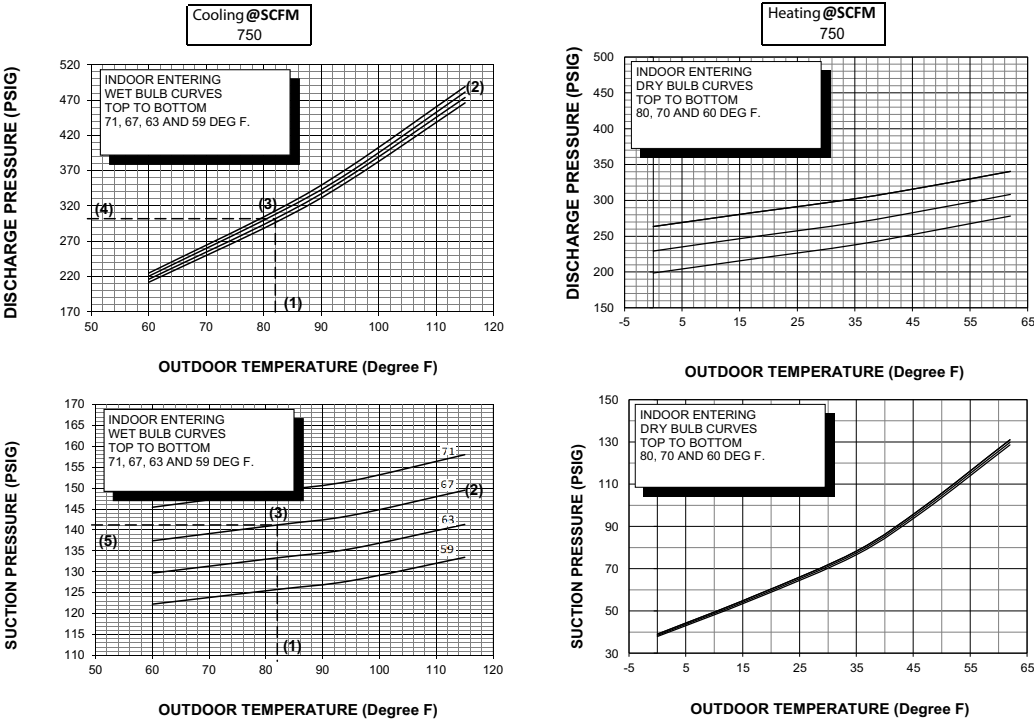
Figure 42. Pressure curves - model 5A6H4030A1
