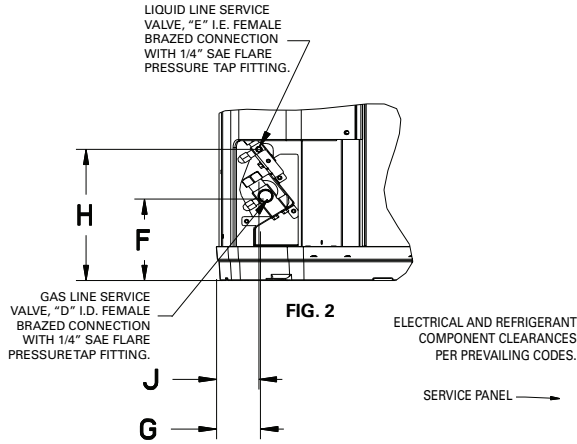
Figure 2. Dimensional drawing
