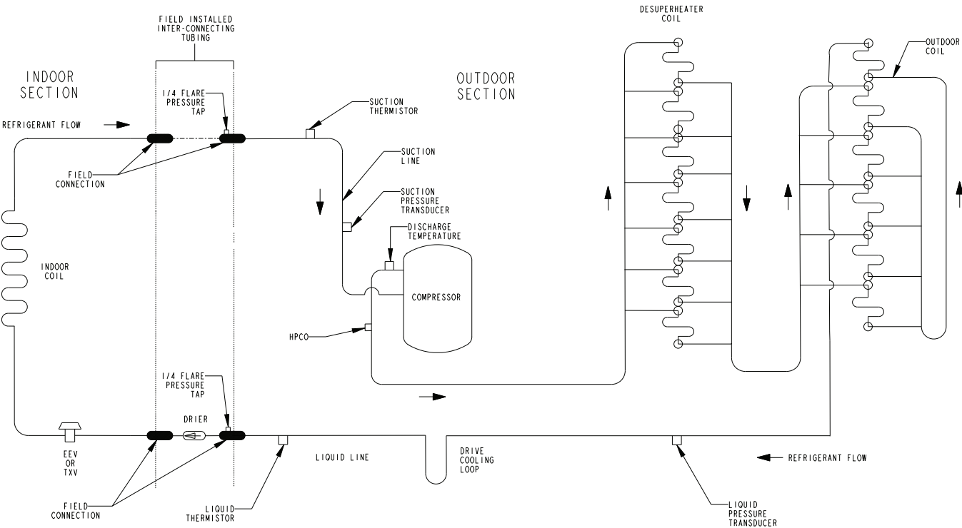
Figure 15. 3-ton, 4-ton, and 5-ton AC (X36, X48, and X60 models)
