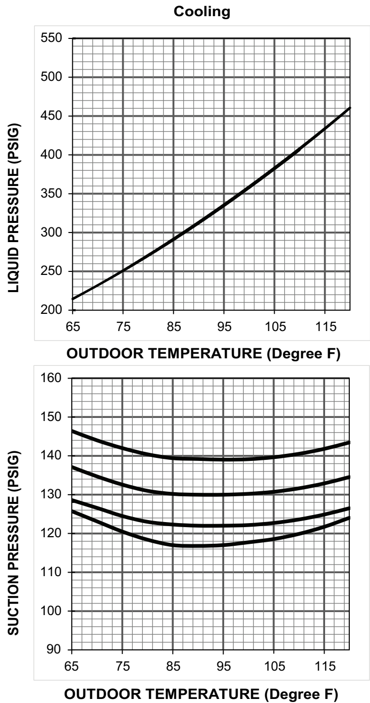
Figure 36. 3 ton AC (X36 model)
