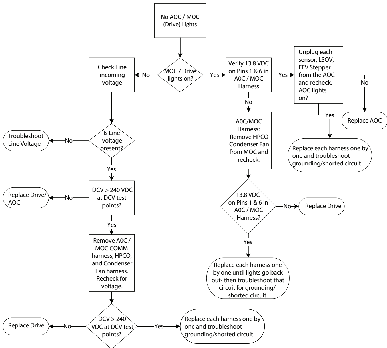
Figure 21. Communication loss flowchart
