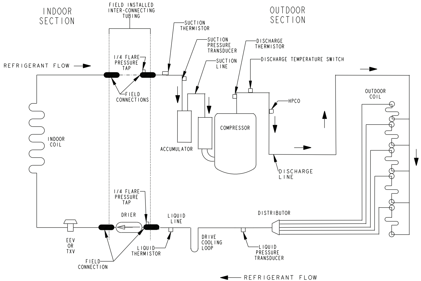
Figure 13. 2-ton AC (X24 model)
