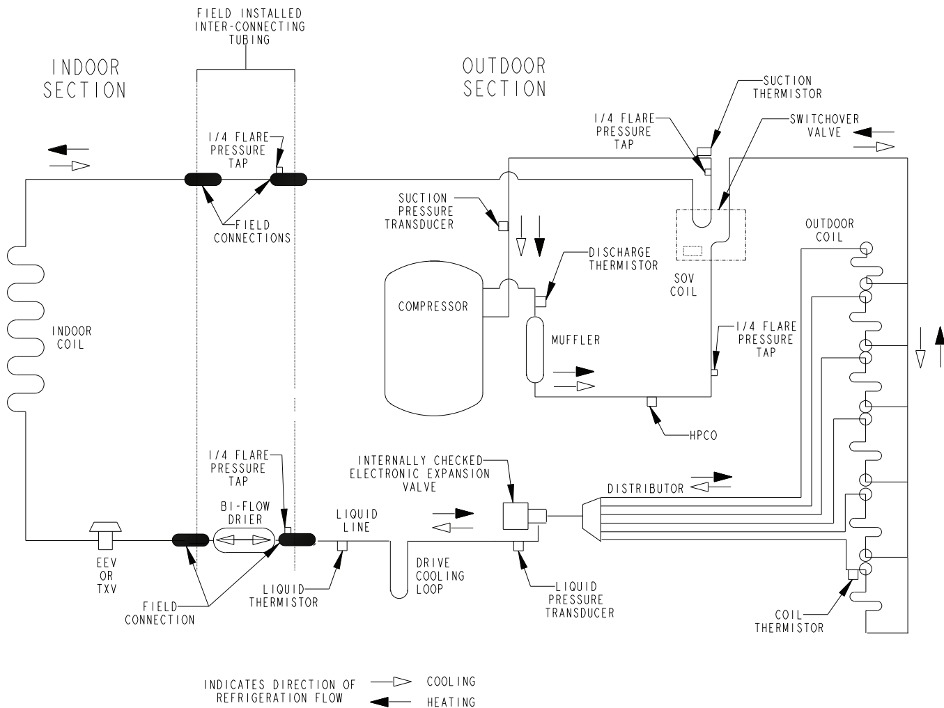
Figure 17. 3-ton HP (X36 model)
