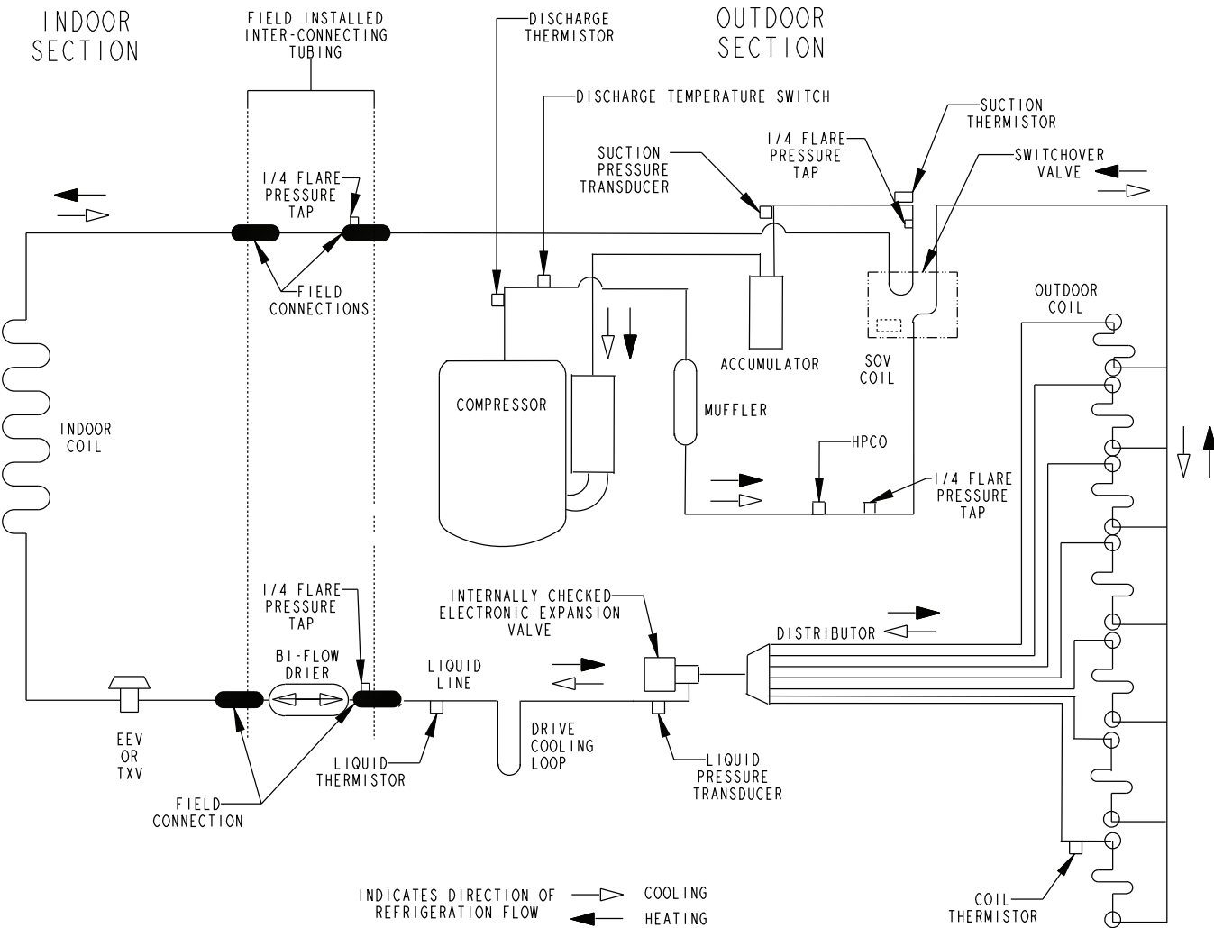
Figure 19. 5-ton HP (X60 models)
