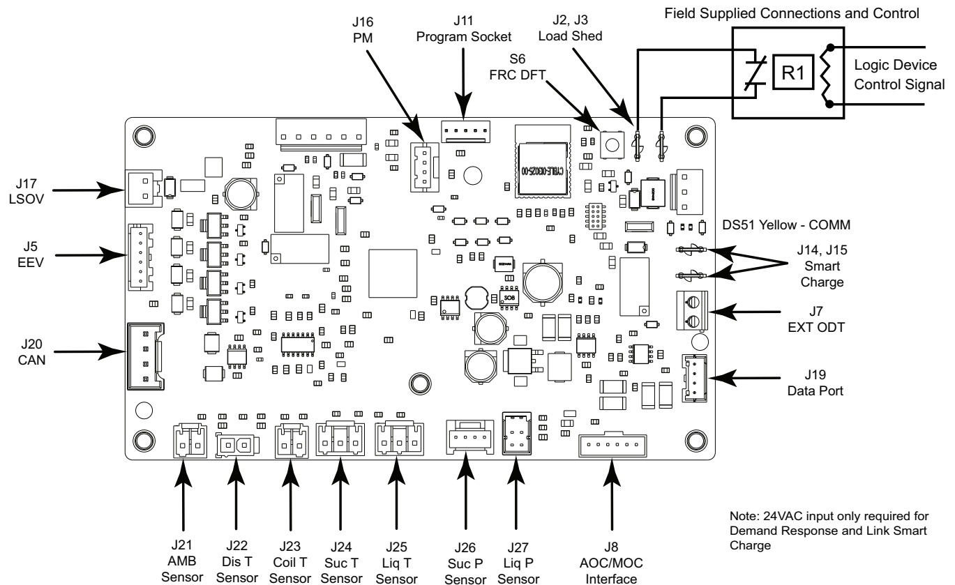
Figure 20. Load shed AOC diagram
