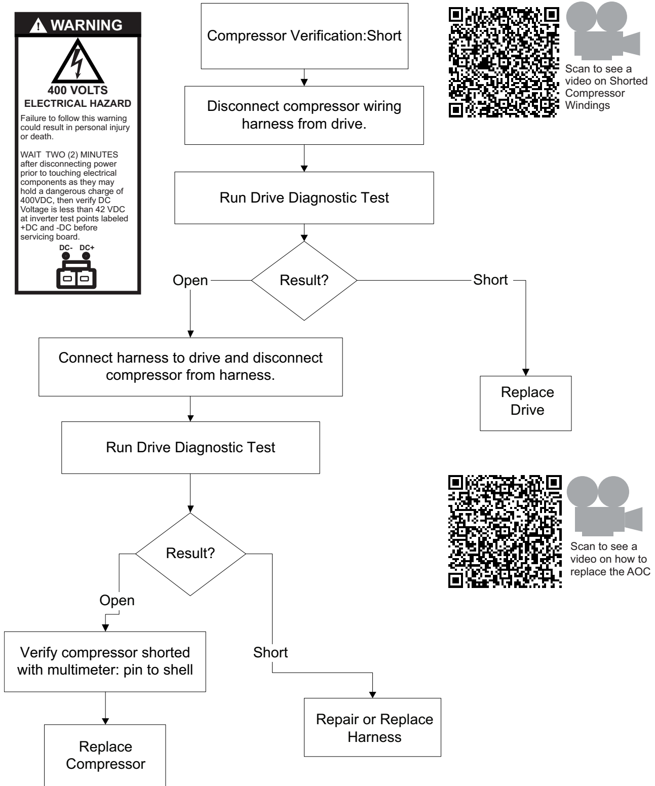
Figure 25. Compressor verification: short flowchart
