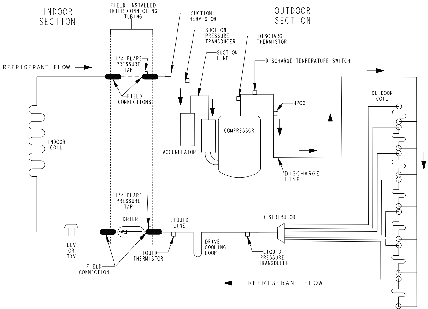
Figure 14. 2-ton AC (X25 model)
