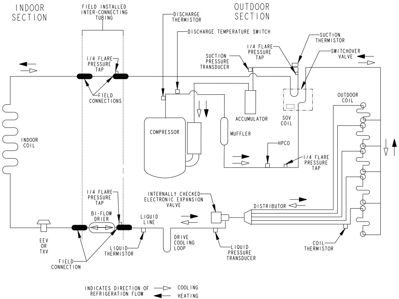
Figure 16. 2-ton HP (X24 model)
