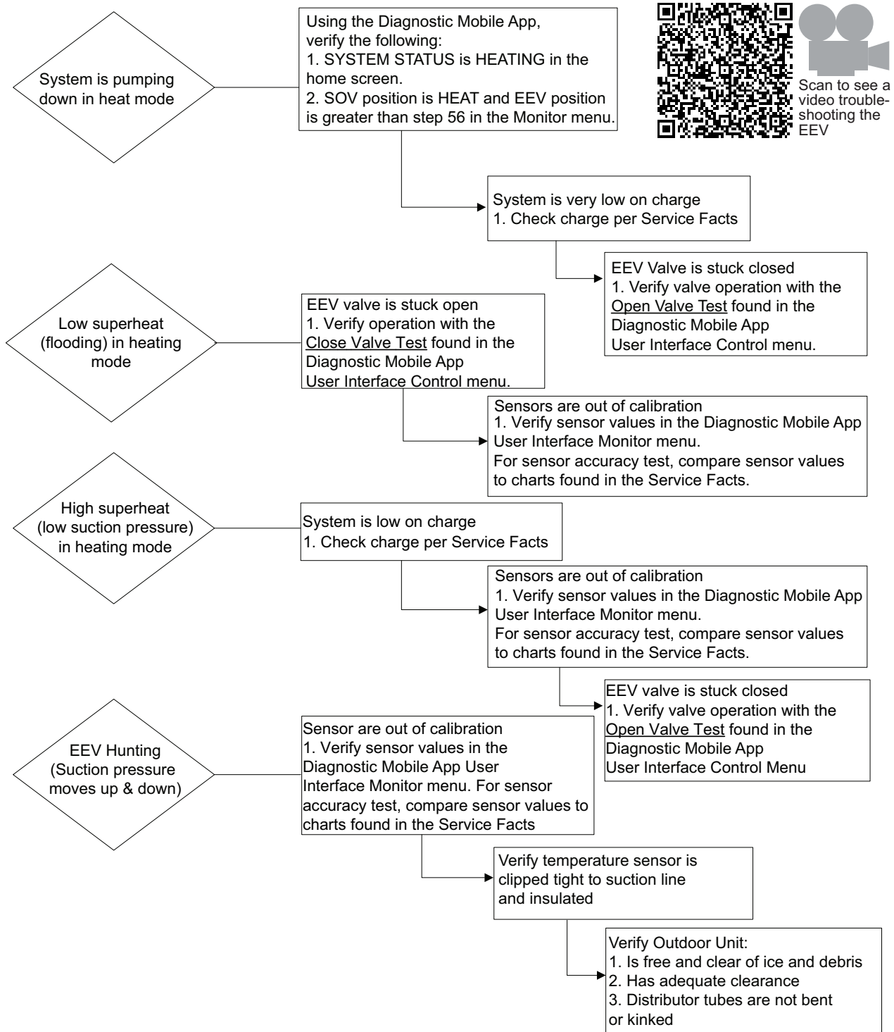
Figure 29. EEV troubleshooting flowchart
