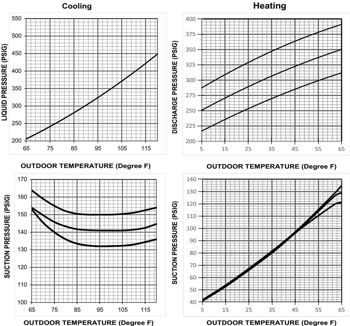
Figure 31. 2 ton HP (X24 model)
