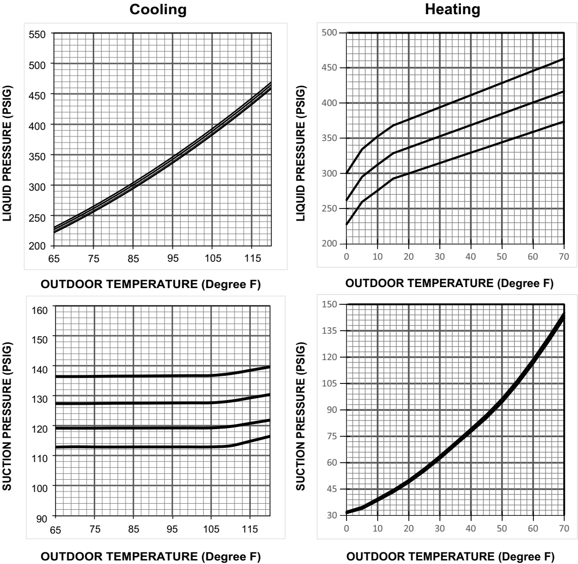
Figure 34. 5 ton HP (X60 model)
