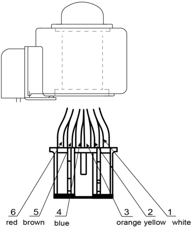
Figure 28. Stepper motor troubleshooting
