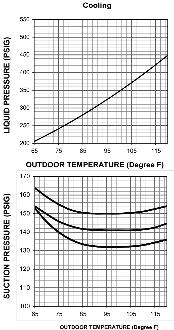
Figure 35. 2 ton AC (X24 and X25 models)
