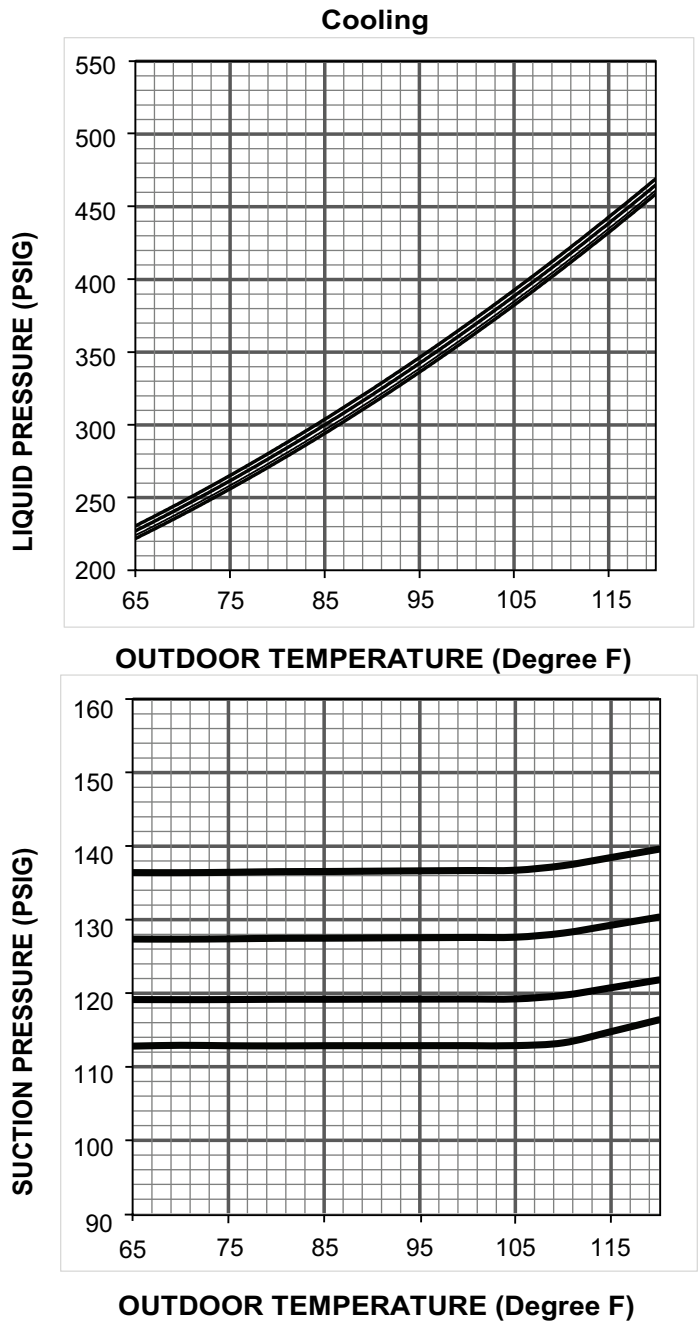
Figure 38. 5 ton AC (X60 model)
