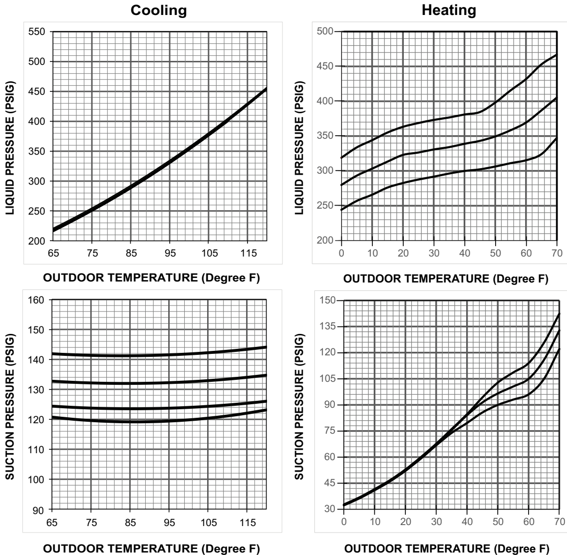
Figure 33. 4 ton HP (X48 model)
