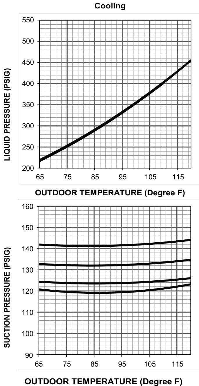
Figure 37. 4 ton AC (X48 model)
