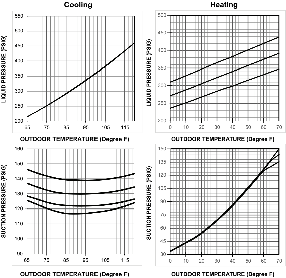
Figure 32. 3 ton HP (X36 model)
