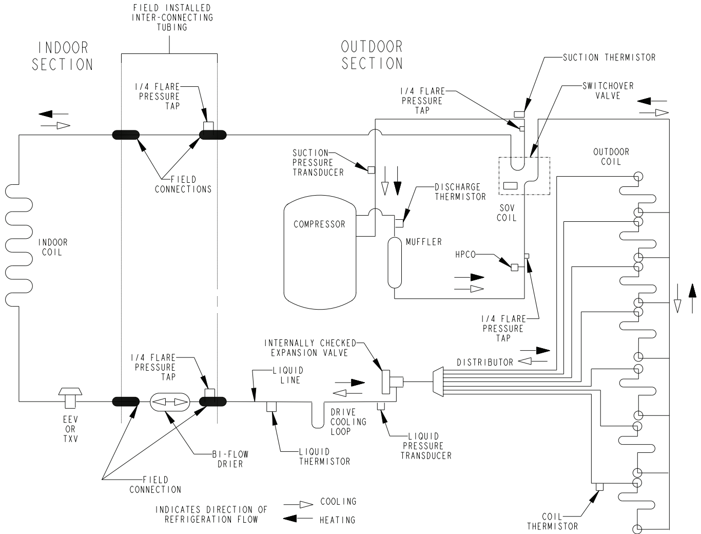
Figure 18. 4-ton HP (X48 model)
