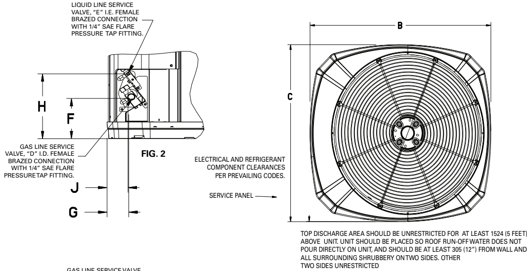
Figure 2. Dimensional drawing
