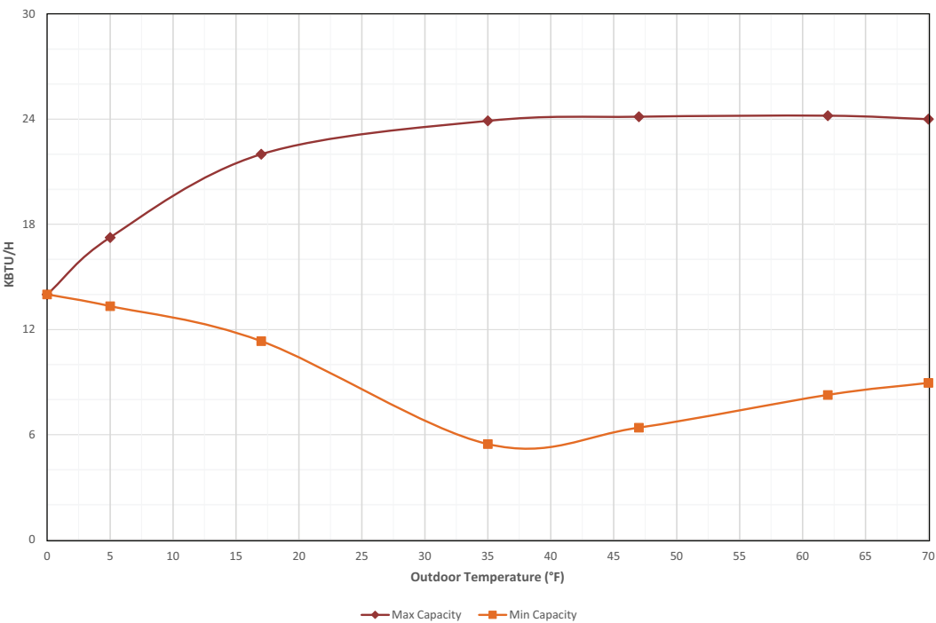
Figure 3. 2-ton heating capacity – model 5A6V8X24A1
