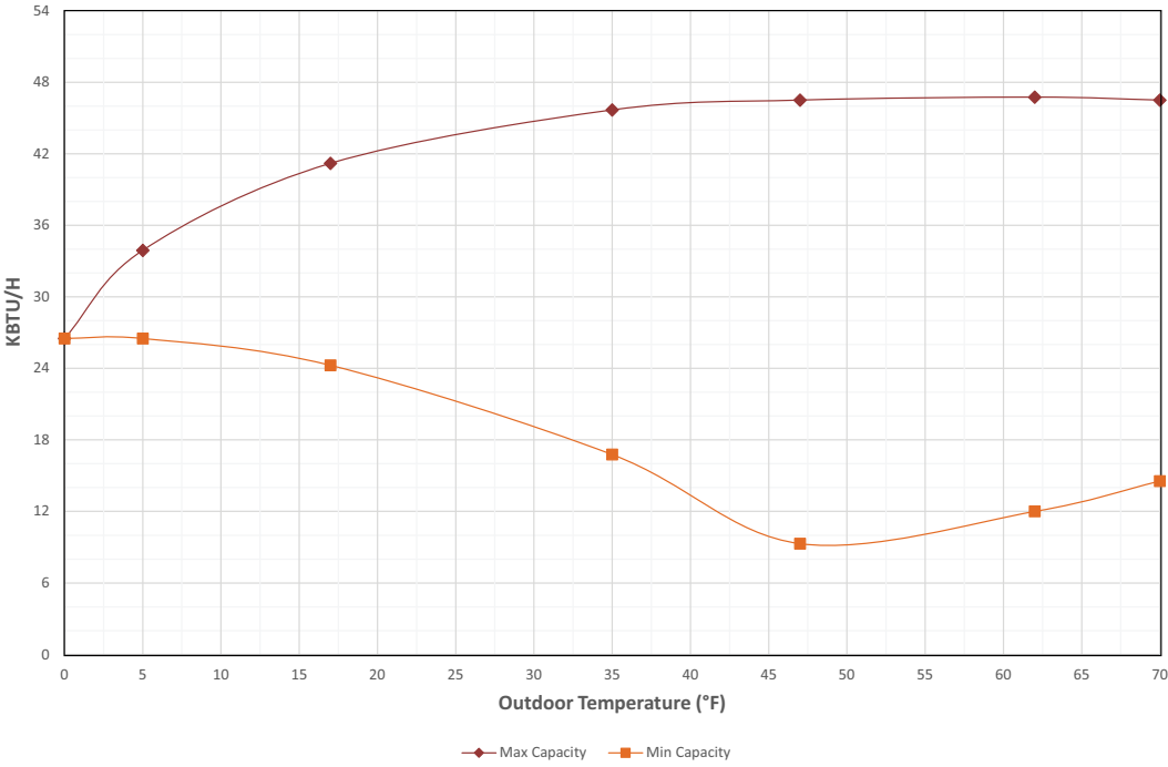
Figure 5. 4-ton heating capacity – model 5A6V8X48A1
