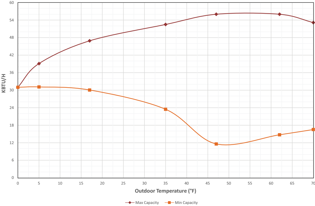
Figure 6. 5-ton heating capacity – model 5A6V8X60A1
