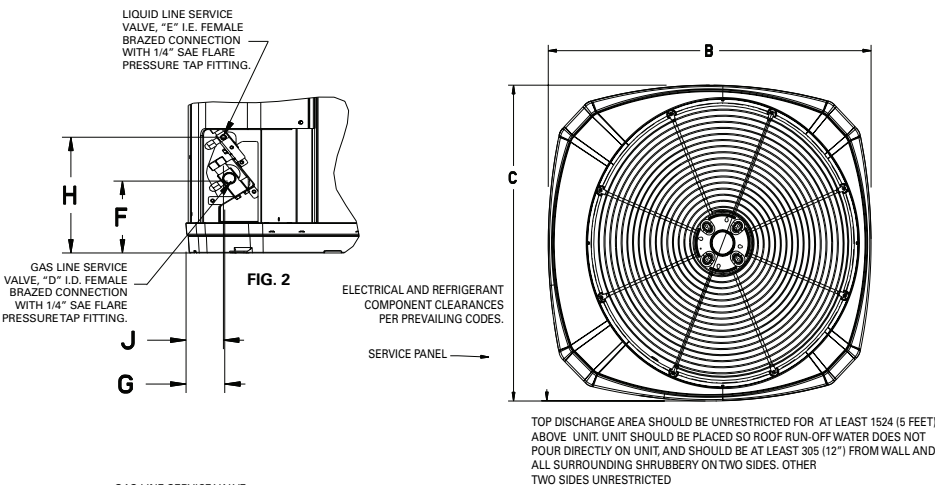
Figure 2. Dimensional drawing
