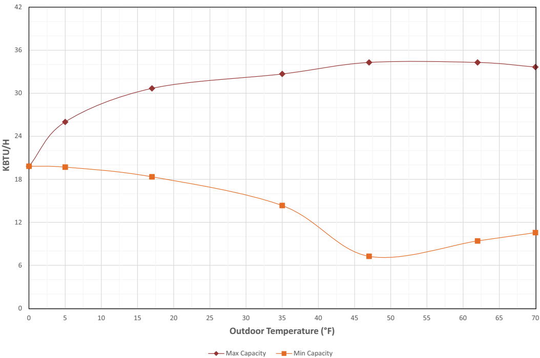
Figure 4. 3-ton heating capacity – model 5A6V8X36A1
