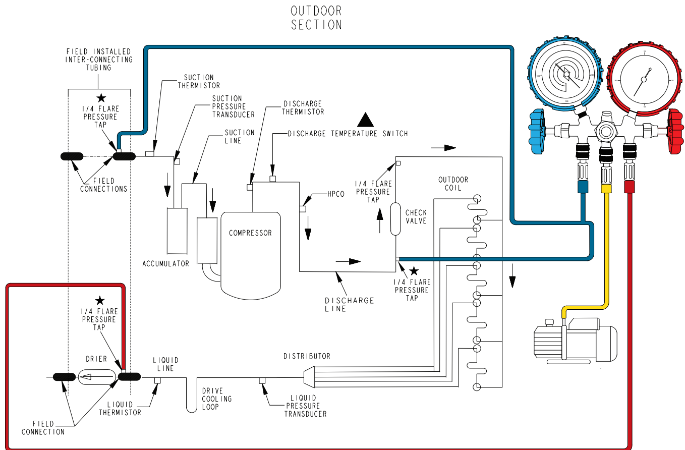
Figure 21. Evacuating Outdoor Unit
